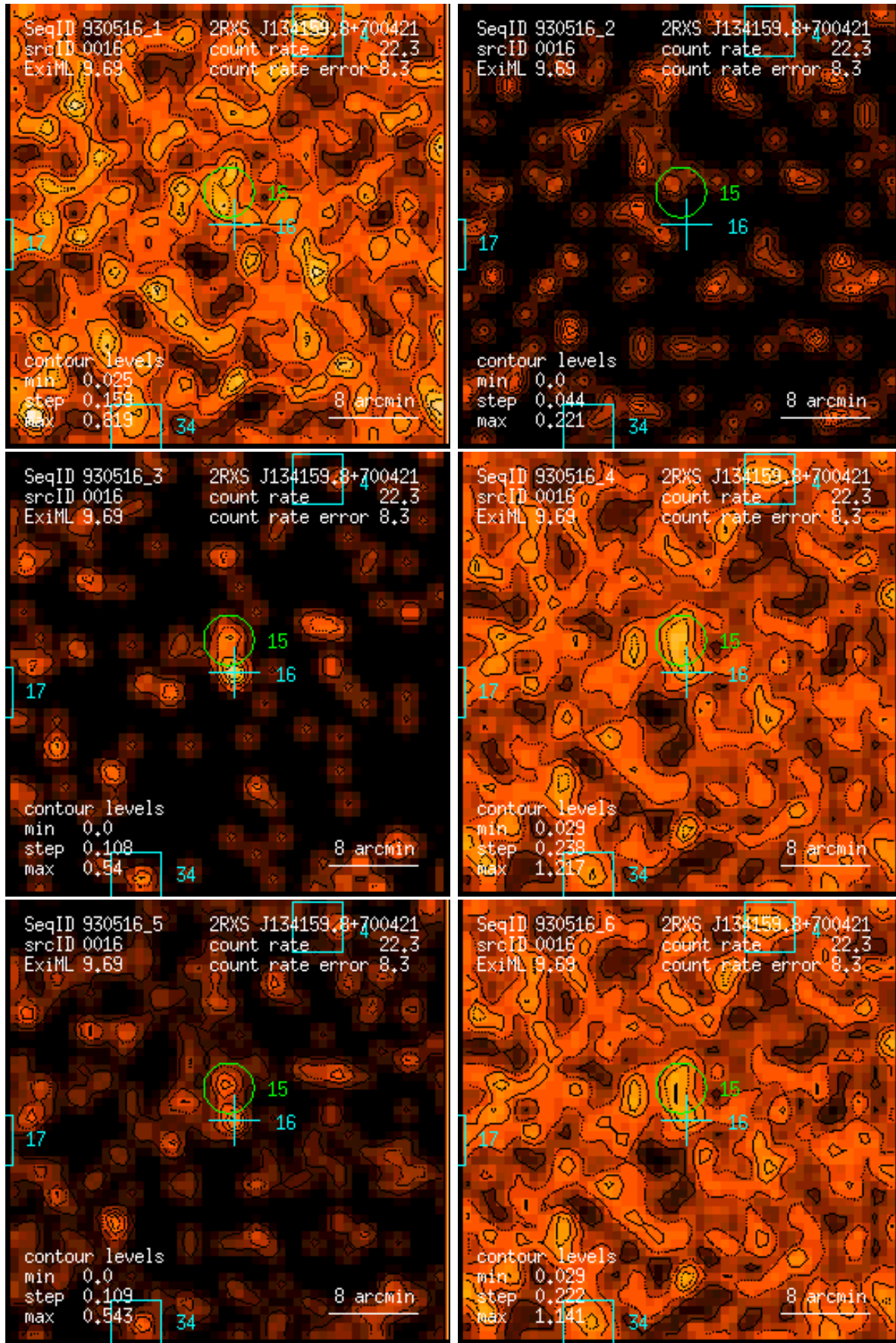
Figure 16: RASS 930516: detection 0016: band rate images, Gaussian filter: (1) PSPC channels 11 – 41, (2) 52 – 90, (3) 91 – 201, (4) 11 – 235, (5) 52 – 201, (6) 11 – 201. Broad band rates in counts/ks. Band rate contour levels in counts/ks/arcmin 2 .
