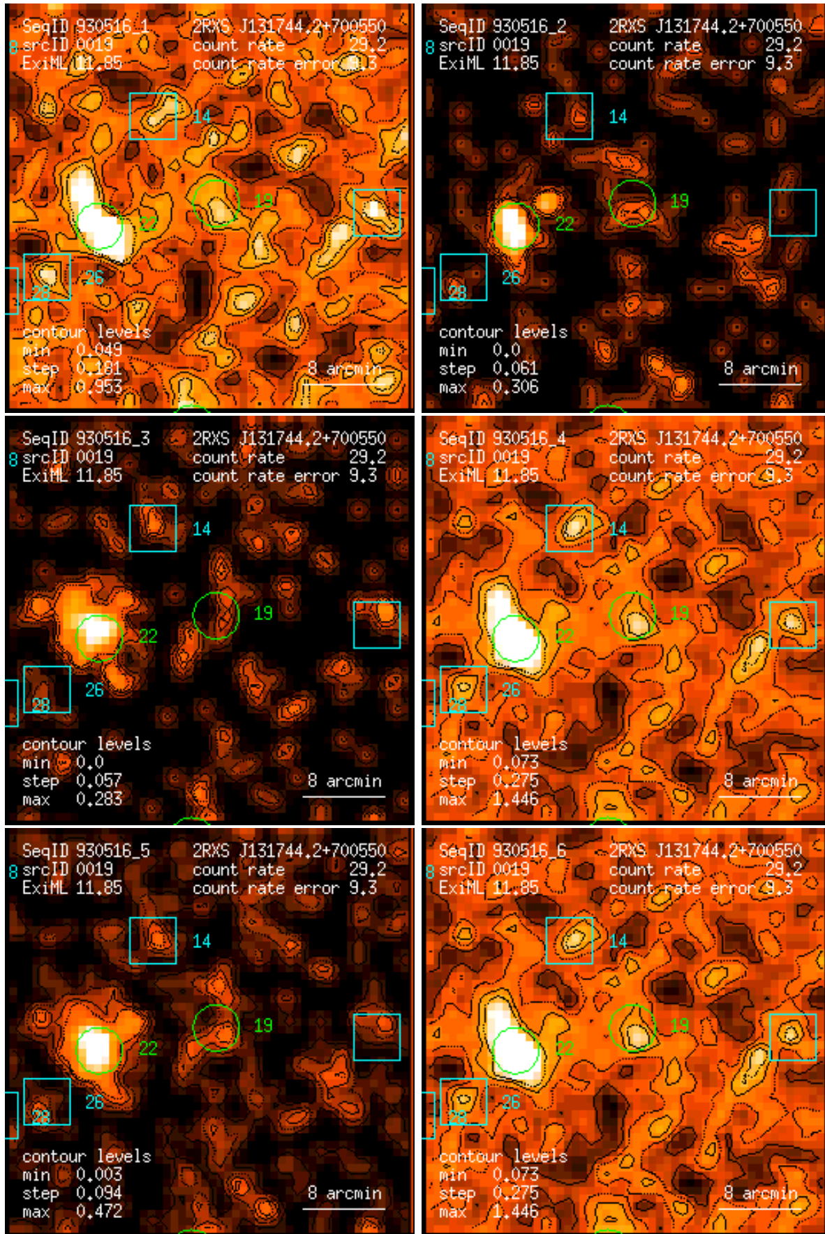
Figure 19: RASS 930516: detection 0019: band rate images, Gaussian filter: (1) PSPC channels 11 – 41, (2) 52 – 90, (3) 91 – 201, (4) 11 – 235, (5) 52 – 201, (6) 11 – 201. Broad band rates in counts/ks. Band rate contour levels in counts/ks/arcmin 2 .
