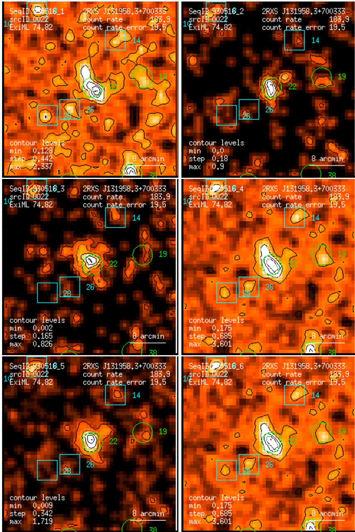
Figure 22: RASS 930516: detection 0022: band rate images, Gaussian filter: (1) PSPC channels 11 – 41, (2) 52 – 90, (3) 91 – 201, (4) 11 – 235, (5) 52 – 201, (6) 11 – 201. Broad band rates in counts/ks. Band rate contour levels in counts/ks/arcmin 2 .
