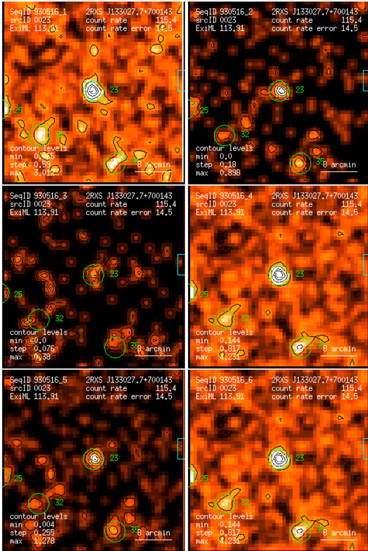
Figure 23: RASS 930516: detection 0023: band rate images, Gaussian filter: (1) PSPC channels 11 – 41, (2) 52 – 90, (3) 91 – 201, (4) 11 – 235, (5) 52 – 201, (6) 11 – 201. Broad band rates in counts/ks. Band rate contour levels in counts/ks/arcmin 2 .
