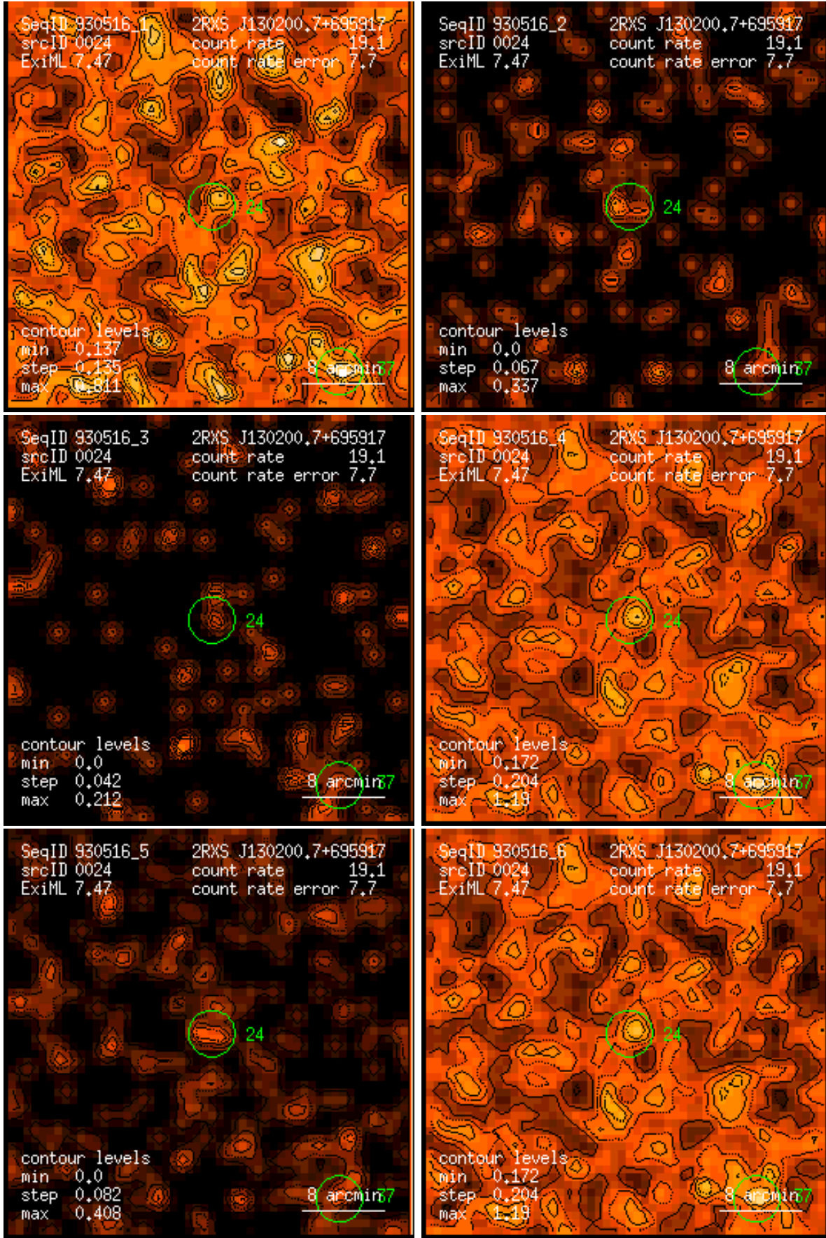
Figure 24: RASS 930516: detection 0024: band rate images, Gaussian filter: (1) PSPC channels 11 – 41, (2) 52 – 90, (3) 91 – 201, (4) 11 – 235, (5) 52 – 201, (6) 11 – 201. Broad band rates in counts/ks. Band rate contour levels in counts/ks/arcmin 2 .
