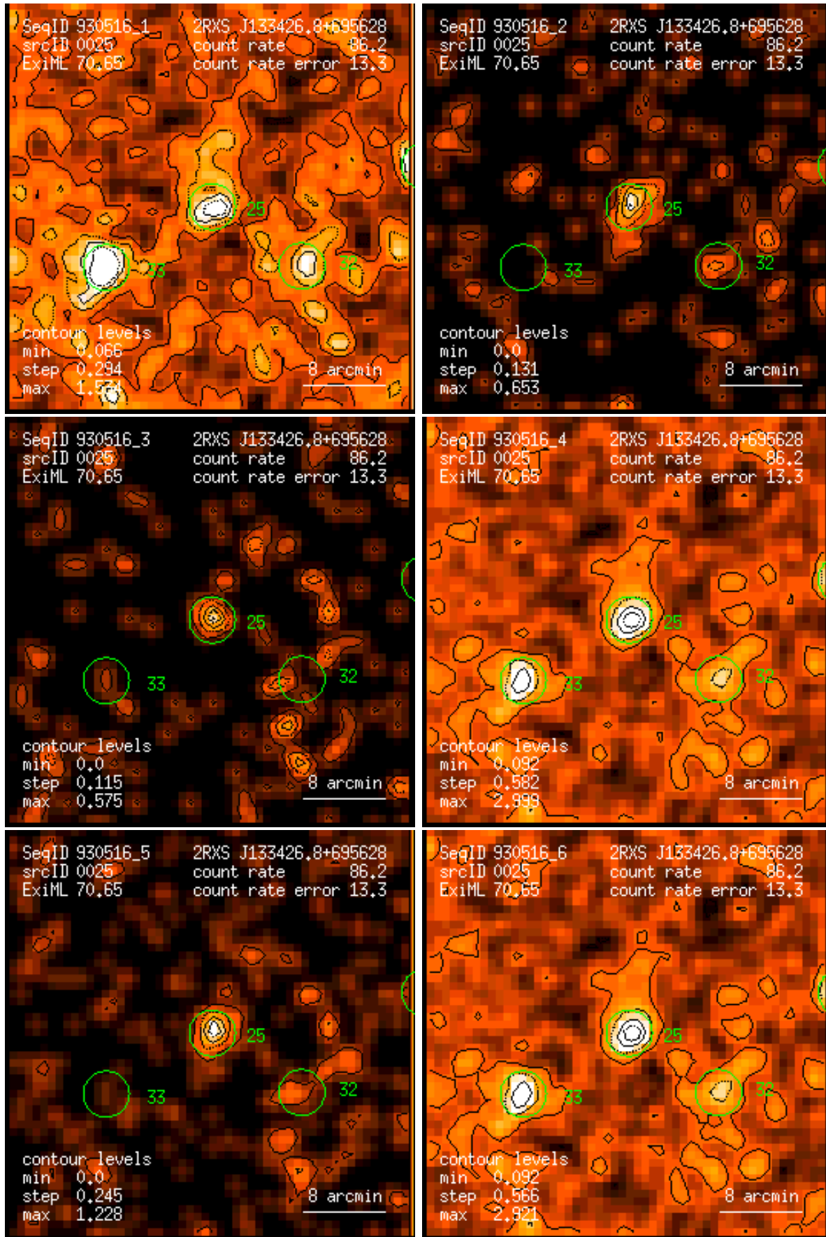
Figure 25: RASS 930516: detection 0025: band rate images, Gaussian filter: (1) PSPC channels 11 – 41, (2) 52 – 90, (3) 91 – 201, (4) 11 – 235, (5) 52 – 201, (6) 11 – 201. Broad band rates in counts/ks. Band rate contour levels in counts/ks/arcmin 2 .
