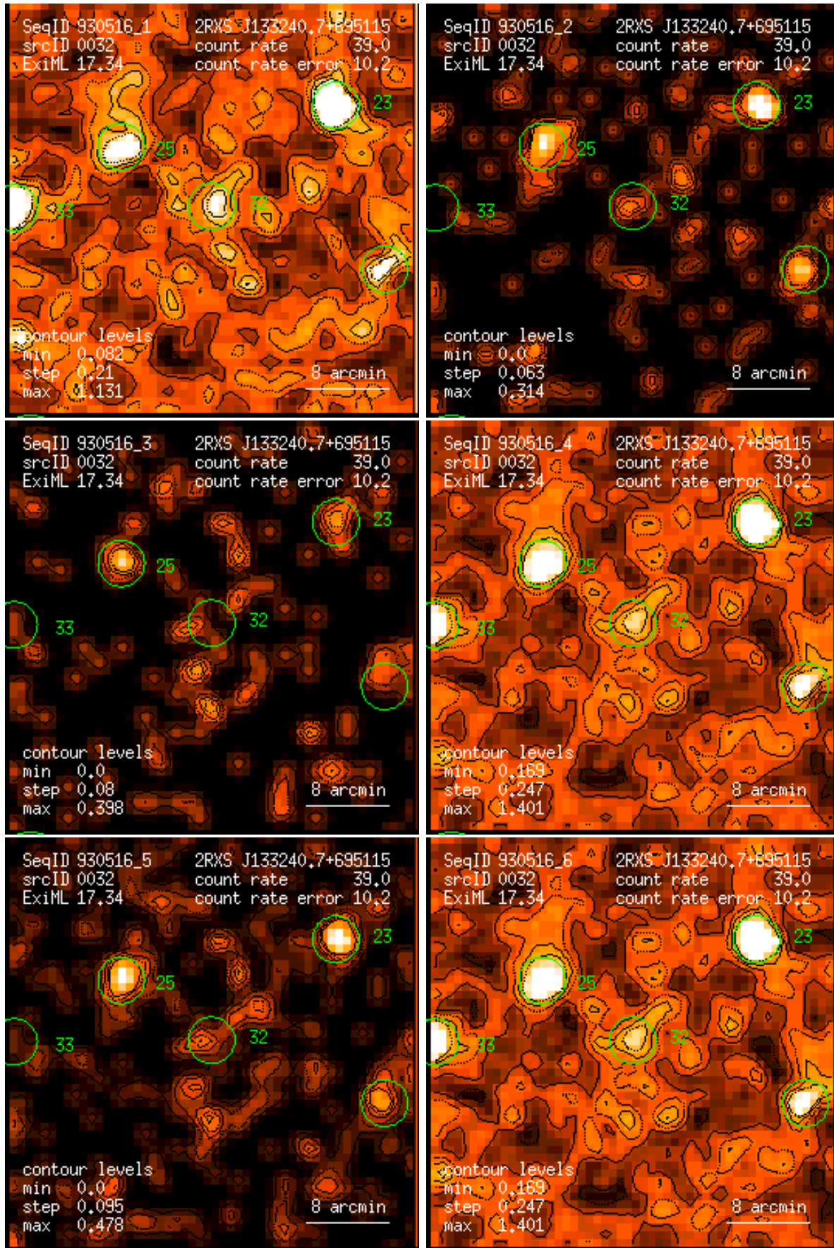
Figure 32: RASS 930516: detection 0032: band rate images, Gaussian filter: (1) PSPC channels 11 – 41, (2) 52 – 90, (3) 91 – 201, (4) 11 – 235, (5) 52 – 201, (6) 11 – 201. Broad band rates in counts/ks. Band rate contour levels in counts/ks/arcmin 2 .
