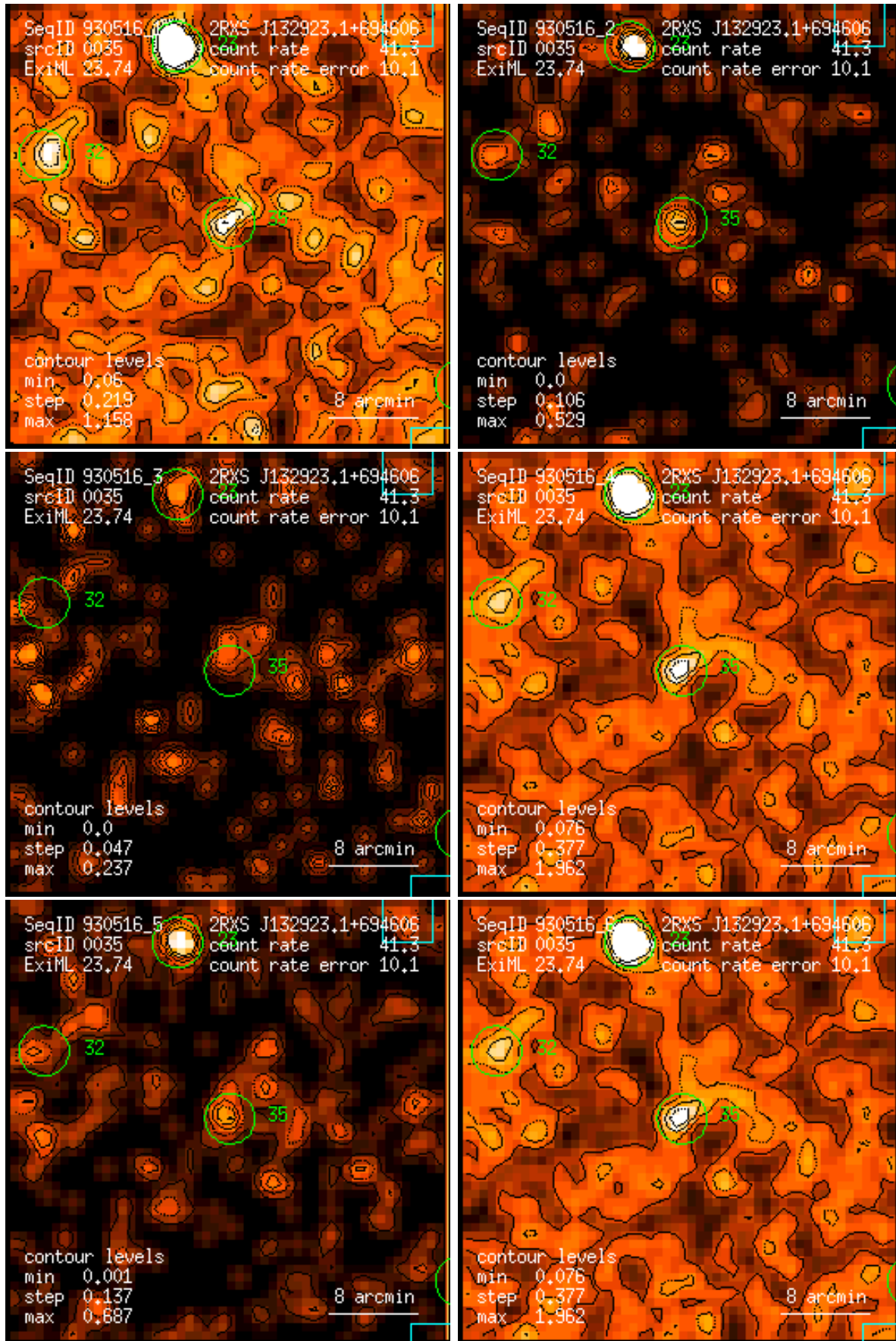
Figure 35: RASS 930516: detection 0035: band rate images, Gaussian filter: (1) PSPC channels 11 – 41, (2) 52 – 90, (3) 91 – 201, (4) 11 – 235, (5) 52 – 201, (6) 11 – 201. Broad band rates in counts/ks. Band rate contour levels in counts/ks/arcmin 2 .
