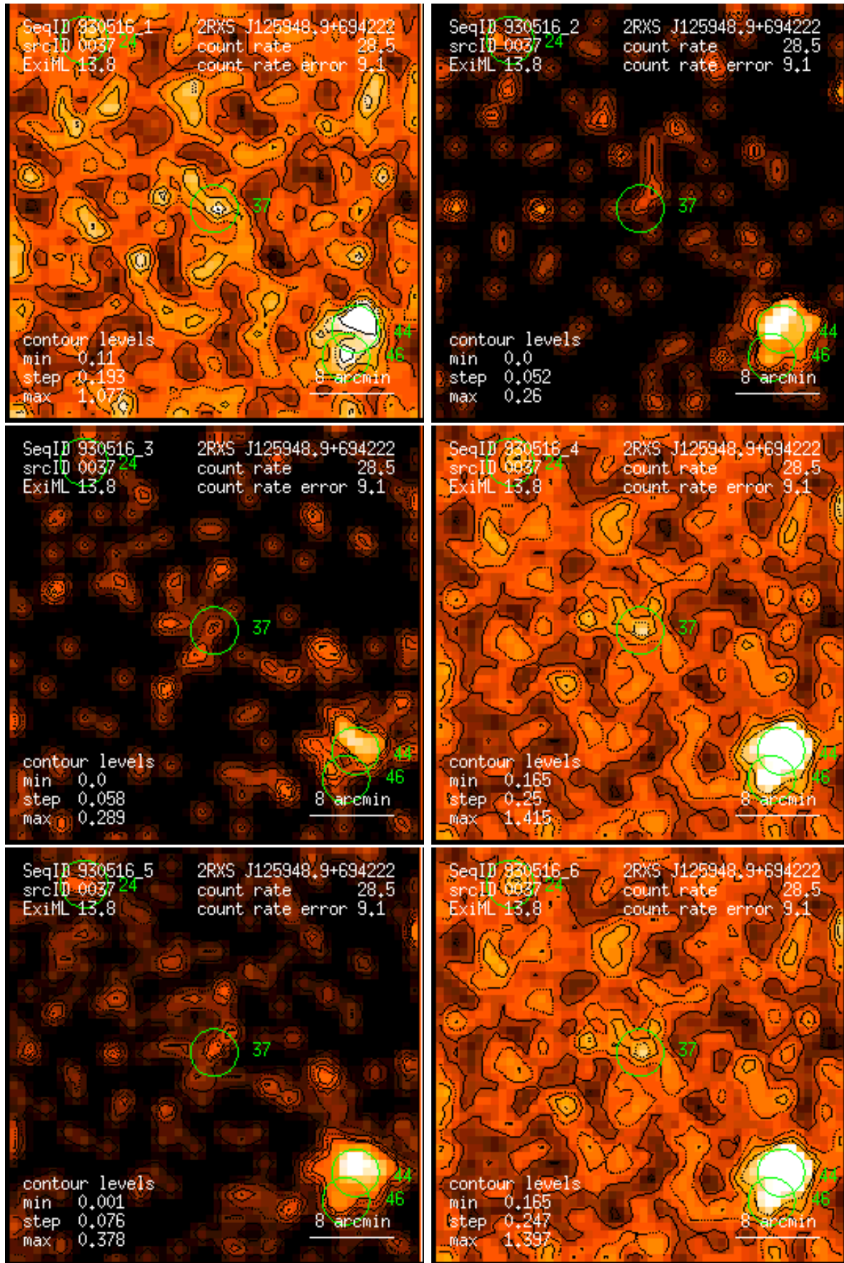
Figure 37: RASS 930516: detection 0037: band rate images, Gaussian filter: (1) PSPC channels 11 – 41, (2) 52 – 90, (3) 91 – 201, (4) 11 – 235, (5) 52 – 201, (6) 11 – 201. Broad band rates in counts/ks. Band rate contour levels in counts/ks/arcmin 2 .
