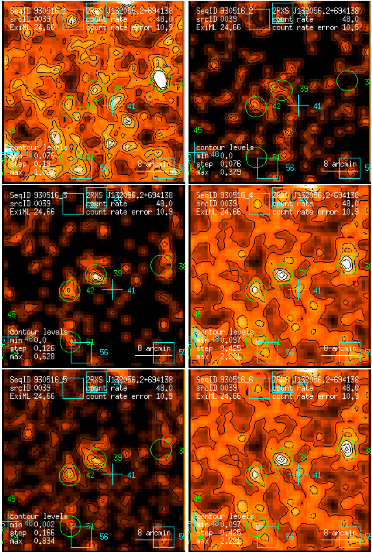
Figure 39: RASS 930516: detection 0039: band rate images, Gaussian filter: (1) PSPC channels 11 – 41, (2) 52 – 90, (3) 91 – 201, (4) 11 – 235, (5) 52 – 201, (6) 11 – 201. Broad band rates in counts/ks. Band rate contour levels in counts/ks/arcmin 2 .
