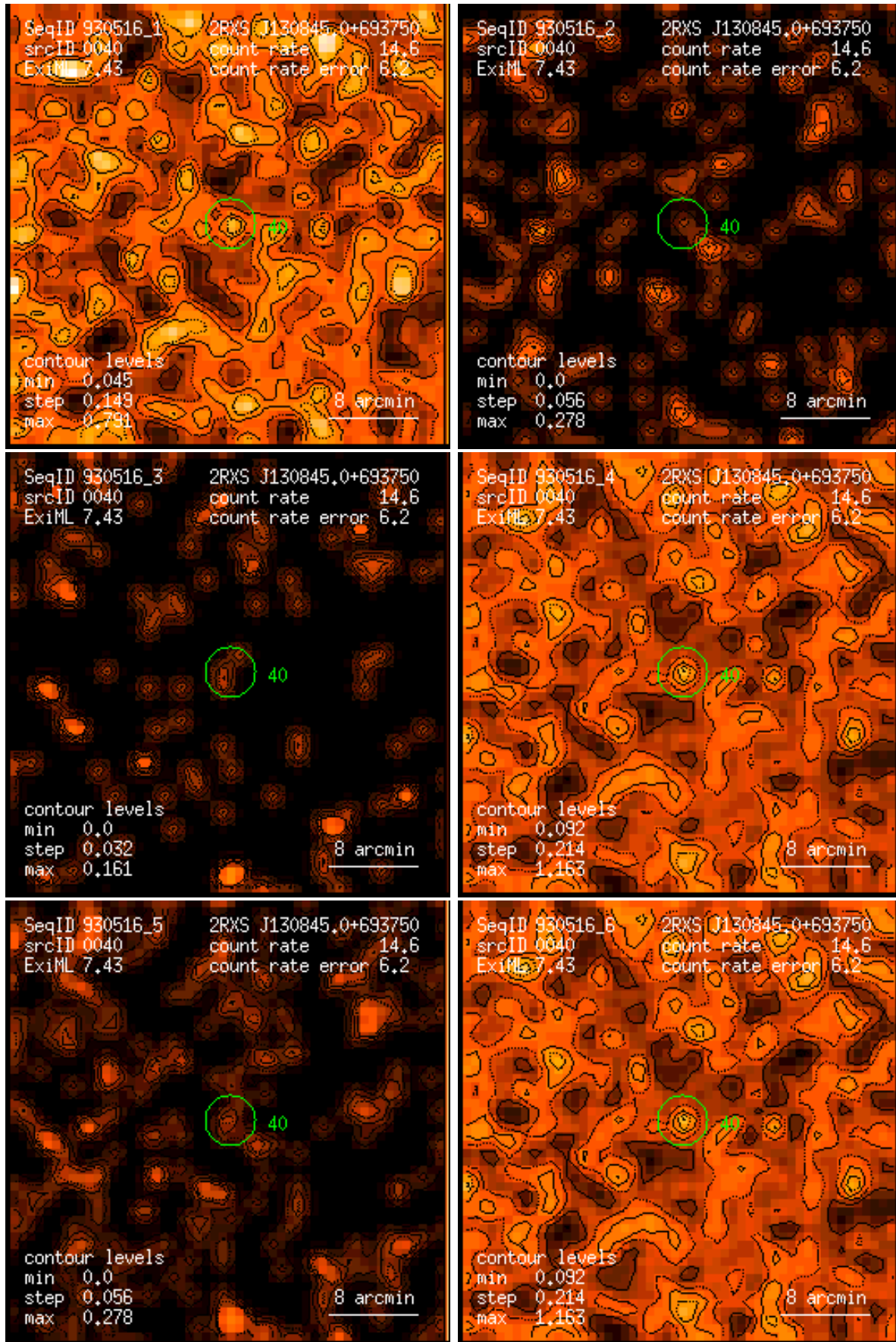
Figure 40: RASS 930516: detection 0040: band rate images, Gaussian filter: (1) PSPC channels 11 – 41, (2) 52 – 90, (3) 91 – 201, (4) 11 – 235, (5) 52 – 201, (6) 11 – 201. Broad band rates in counts/ks. Band rate contour levels in counts/ks/arcmin 2 .
