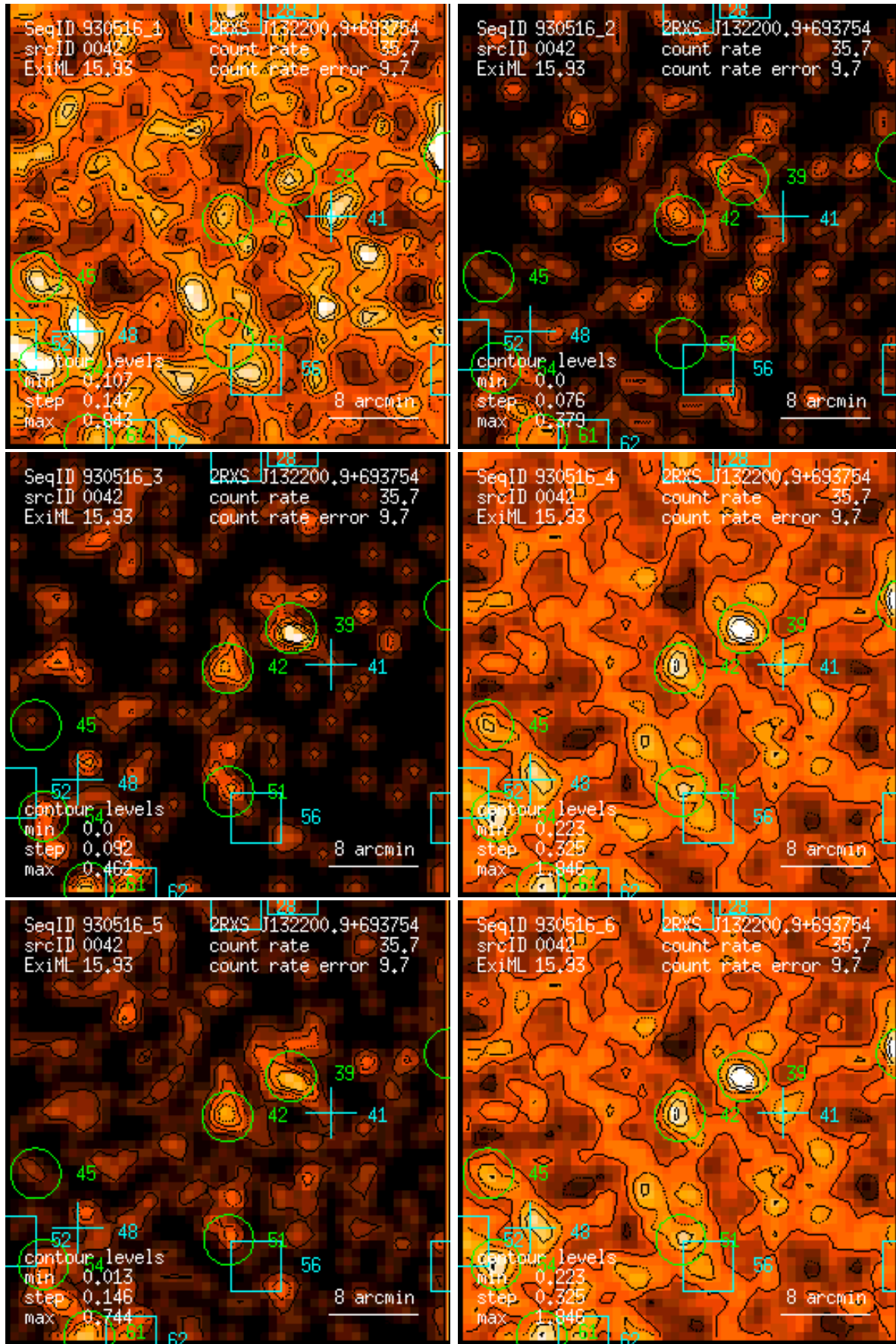
Figure 42: RASS 930516: detection 0042: band rate images, Gaussian filter: (1) PSPC channels 11 – 41, (2) 52 – 90, (3) 91 – 201, (4) 11 – 235, (5) 52 – 201, (6) 11 – 201. Broad band rates in counts/ks. Band rate contour levels in counts/ks/arcmin 2 .
