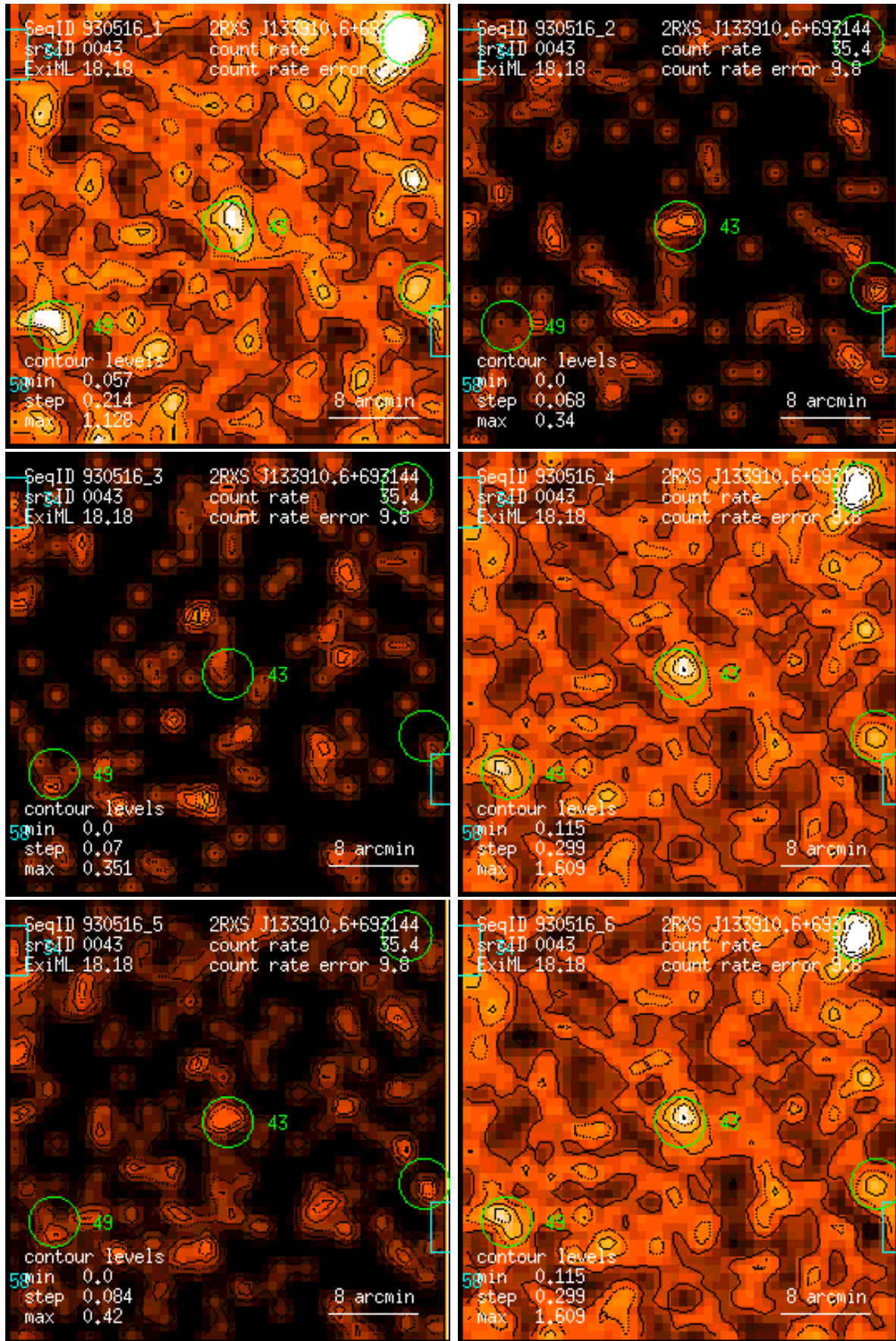
Figure 43: RASS 930516: detection 0043: band rate images, Gaussian filter: (1) PSPC channels 11 – 41, (2) 52 – 90, (3) 91 – 201, (4) 11 – 235, (5) 52 – 201, (6) 11 – 201. Broad band rates in counts/ks. Band rate contour levels in counts/ks/arcmin 2 .
