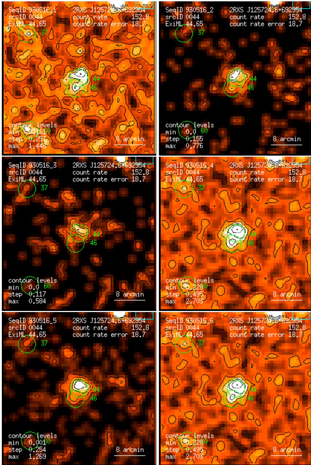
Figure 44: RASS 930516: detection 0044: band rate images, Gaussian filter: (1) PSPC channels 11 – 41, (2) 52 – 90, (3) 91 – 201, (4) 11 – 235, (5) 52 – 201, (6) 11 – 201. Broad band rates in counts/ks. Band rate contour levels in counts/ks/arcmin 2 .
