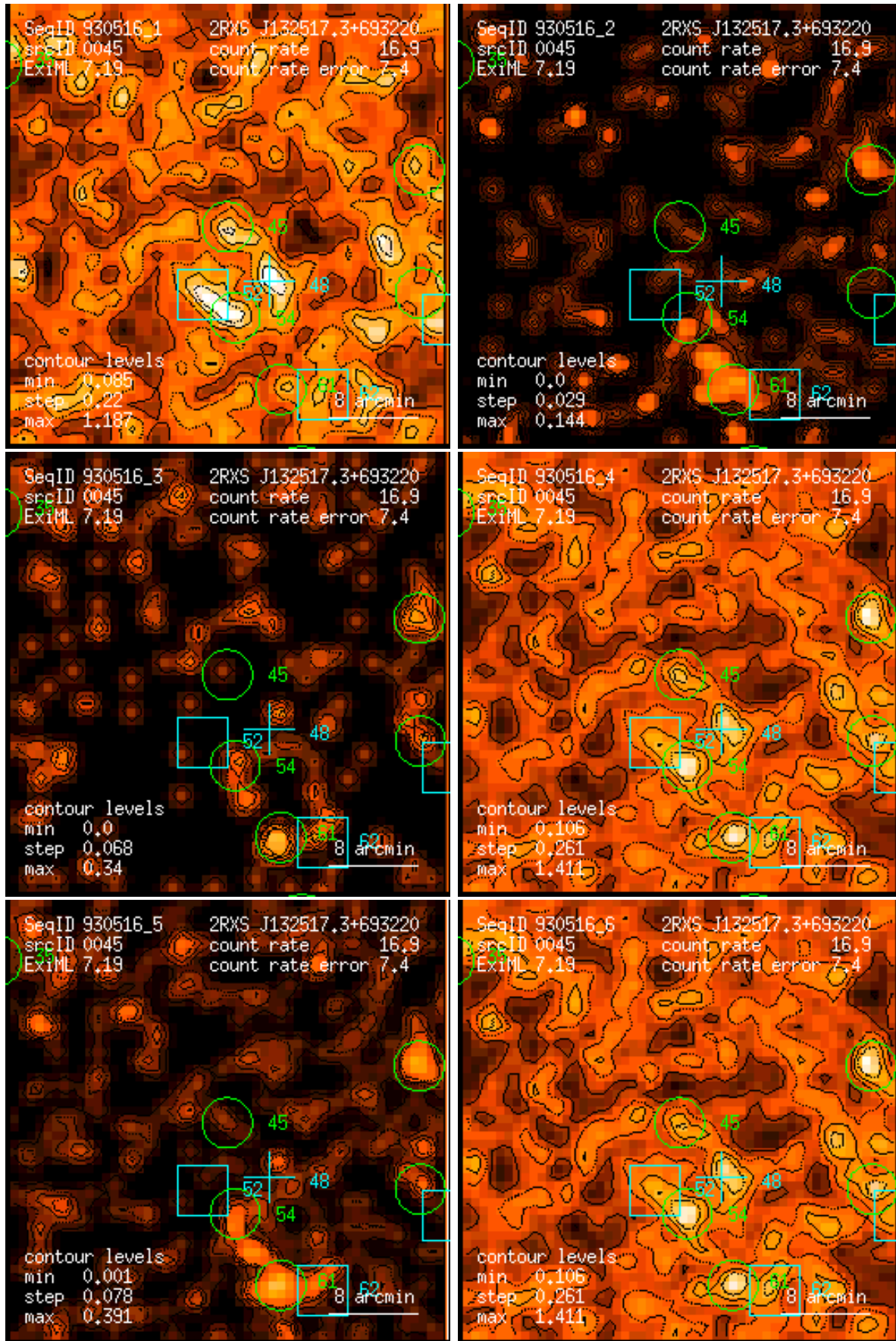
Figure 45: RASS 930516: detection 0045: band rate images, Gaussian filter: (1) PSPC channels 11 – 41, (2) 52 – 90, (3) 91 – 201, (4) 11 – 235, (5) 52 – 201, (6) 11 – 201. Broad band rates in counts/ks. Band rate contour levels in counts/ks/arcmin 2 .
