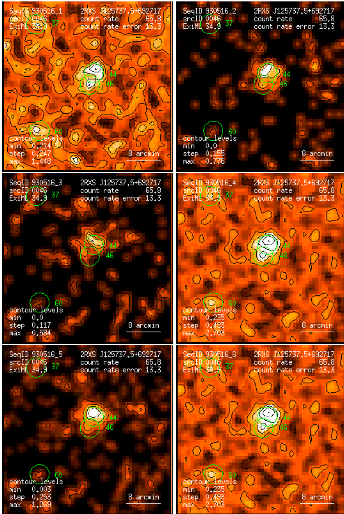
Figure 46: RASS 930516: detection 0046: band rate images, Gaussian filter: (1) PSPC channels 11 – 41, (2) 52 – 90, (3) 91 – 201, (4) 11 – 235, (5) 52 – 201, (6) 11 – 201. Broad band rates in counts/ks. Band rate contour levels in counts/ks/arcmin 2 .
