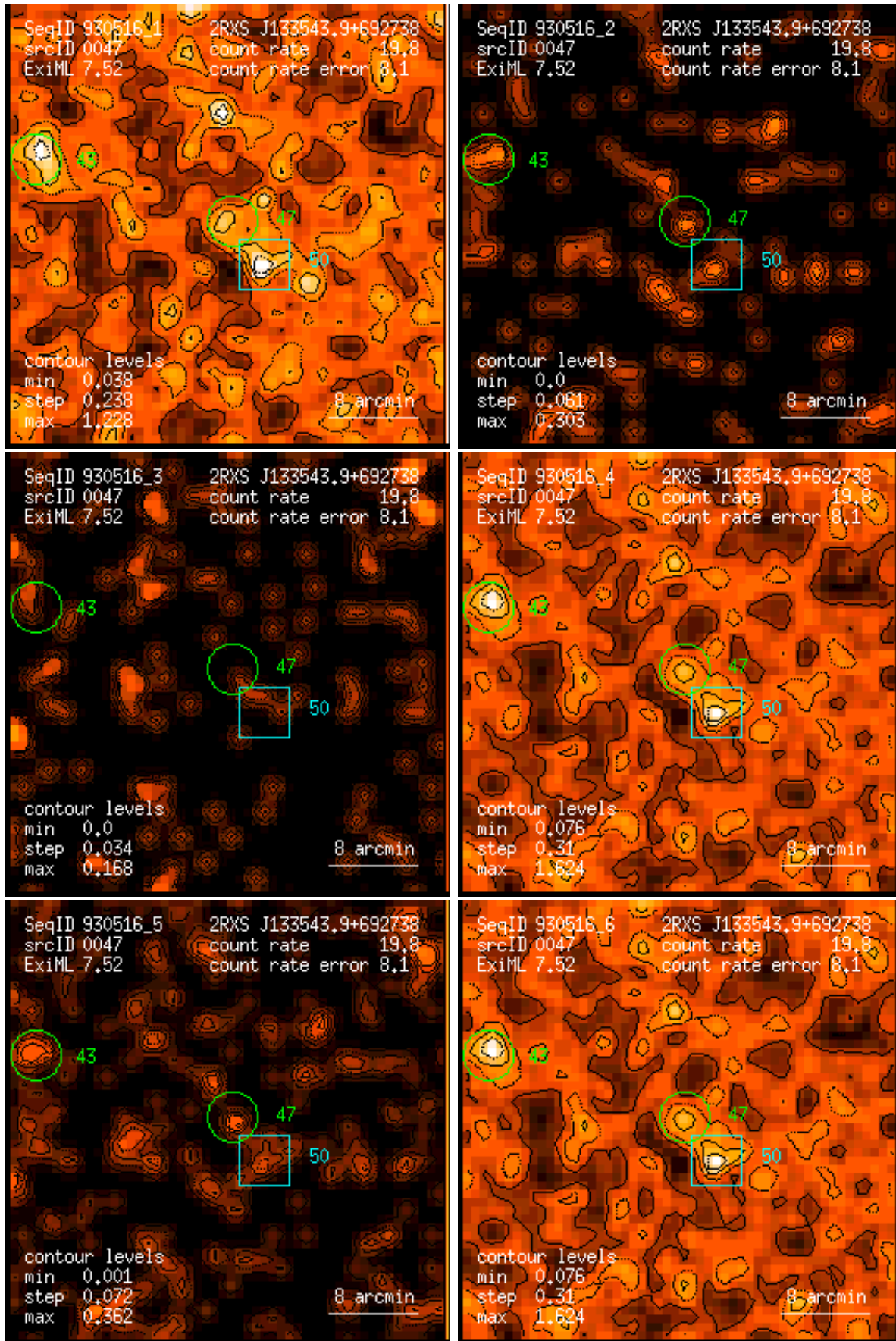
Figure 47: RASS 930516: detection 0047: band rate images, Gaussian filter: (1) PSPC channels 11 – 41, (2) 52 – 90, (3) 91 – 201, (4) 11 – 235, (5) 52 – 201, (6) 11 – 201. Broad band rates in counts/ks. Band rate contour levels in counts/ks/arcmin 2 .
