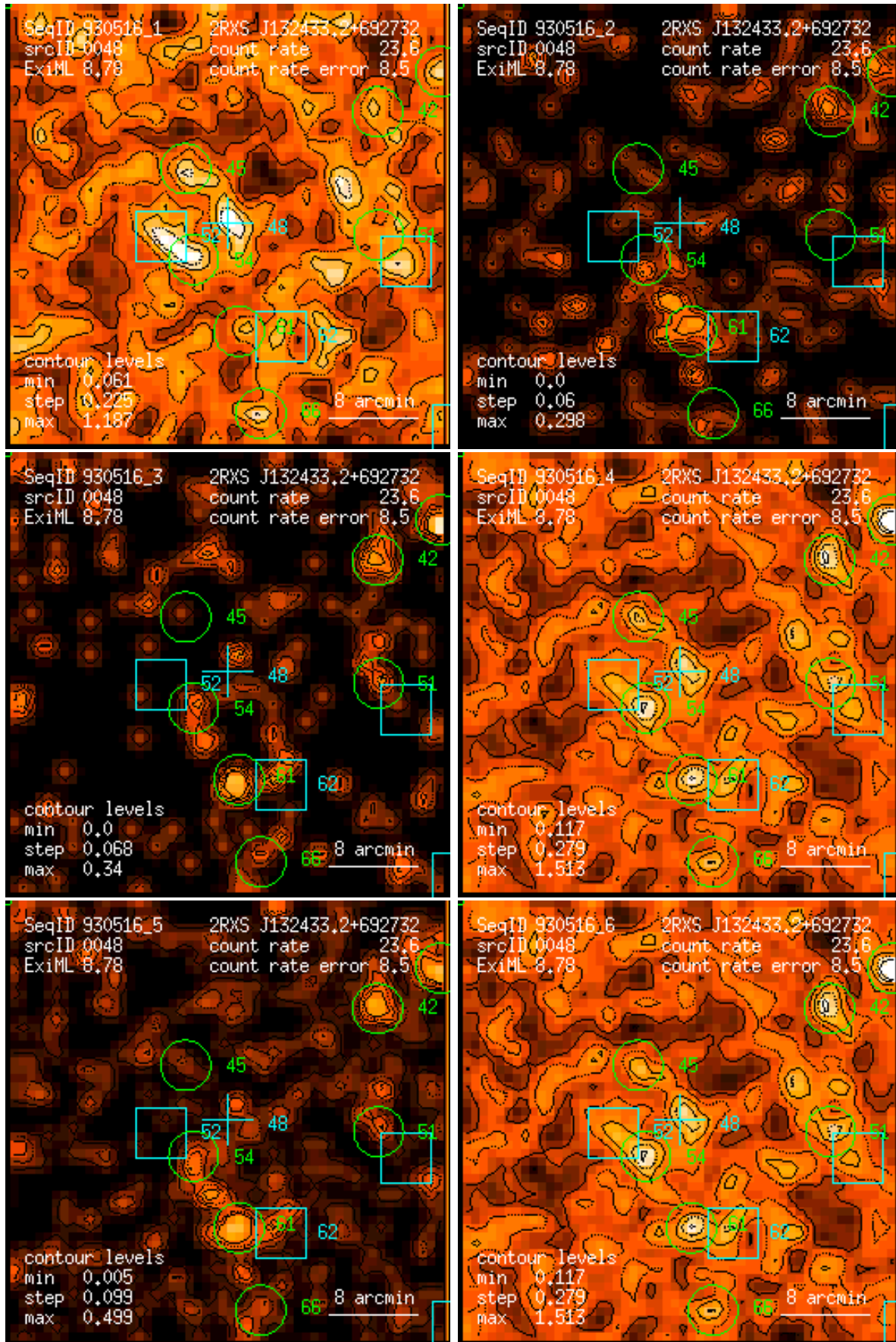
Figure 48: RASS 930516: detection 0048: band rate images, Gaussian filter: (1) PSPC channels 11 – 41, (2) 52 – 90, (3) 91 – 201, (4) 11 – 235, (5) 52 – 201, (6) 11 – 201. Broad band rates in counts/ks. Band rate contour levels in counts/ks/arcmin 2 .
