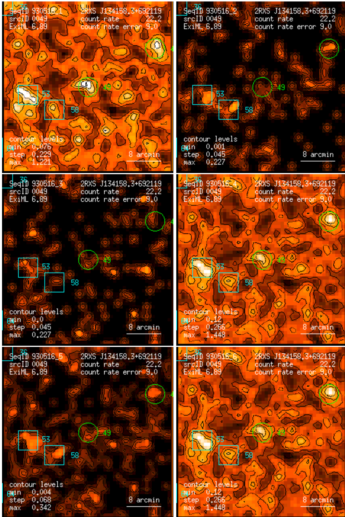
Figure 49: RASS 930516: detection 0049: band rate images, Gaussian filter: (1) PSPC channels 11 – 41, (2) 52 – 90, (3) 91 – 201, (4) 11 – 235, (5) 52 – 201, (6) 11 – 201. Broad band rates in counts/ks. Band rate contour levels in counts/ks/arcmin 2 .
