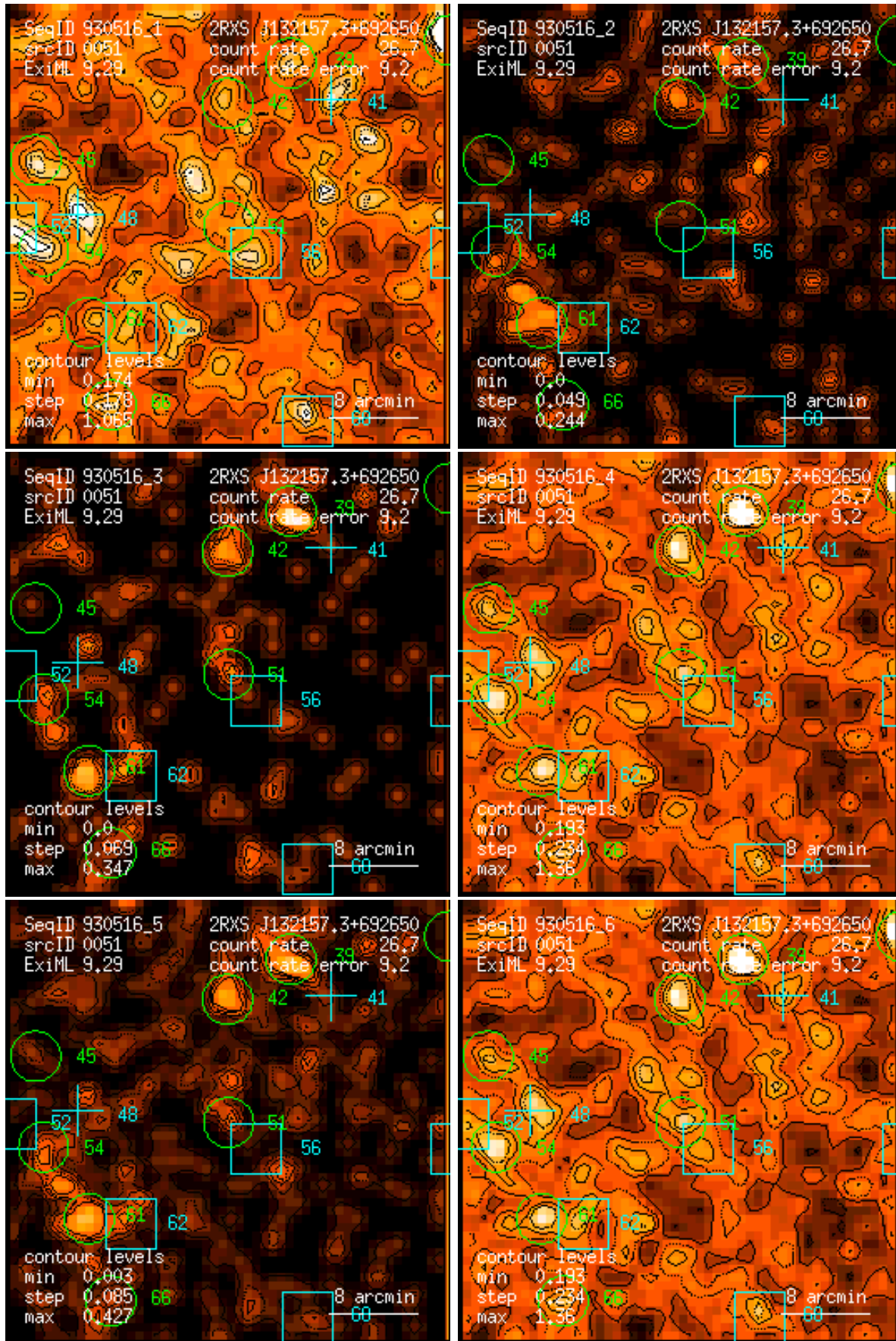
Figure 51: RASS 930516: detection 0051: band rate images, Gaussian filter: (1) PSPC channels 11 – 41, (2) 52 – 90, (3) 91 – 201, (4) 11 – 235, (5) 52 – 201, (6) 11 – 201. Broad band rates in counts/ks. Band rate contour levels in counts/ks/arcmin 2 .
