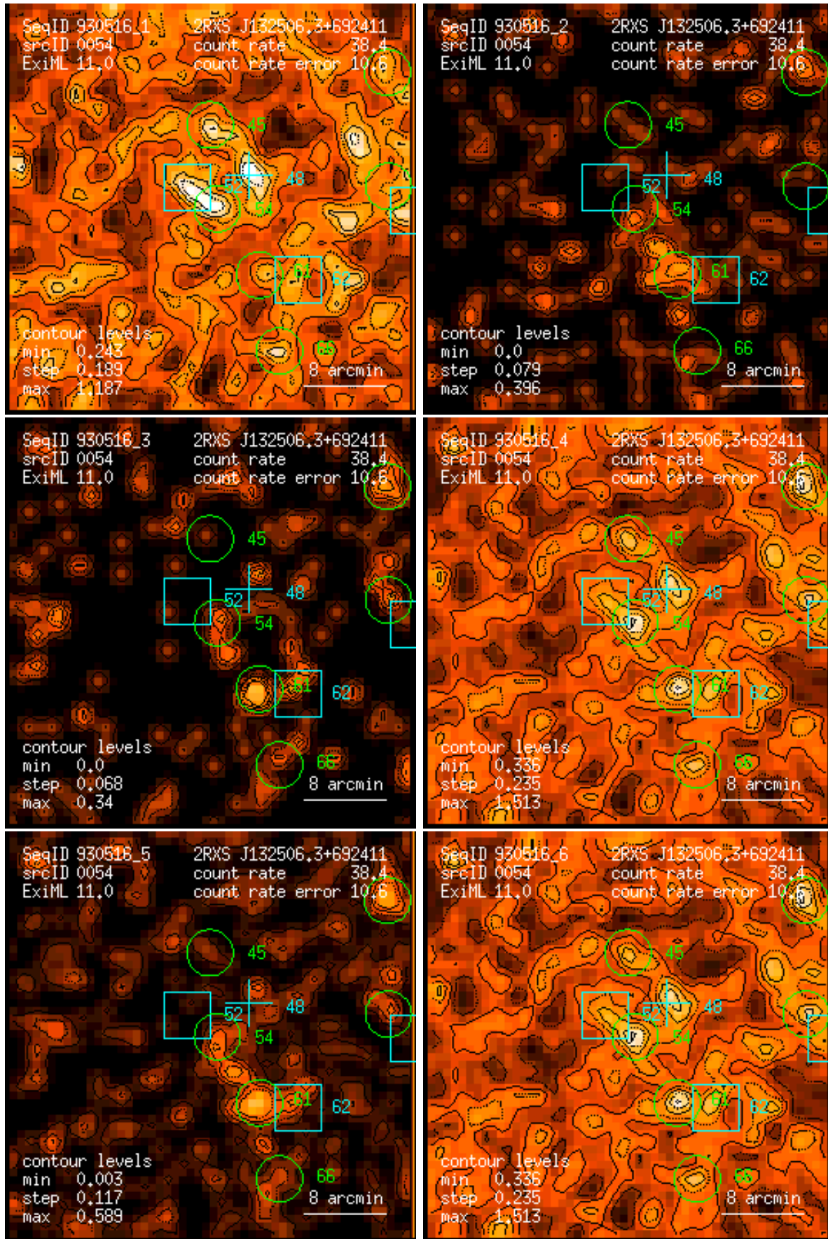
Figure 54: RASS 930516: detection 0054: band rate images, Gaussian filter: (1) PSPC channels 11 – 41, (2) 52 – 90, (3) 91 – 201, (4) 11 – 235, (5) 52 – 201, (6) 11 – 201. Broad band rates in counts/ks. Band rate contour levels in counts/ks/arcmin 2 .
