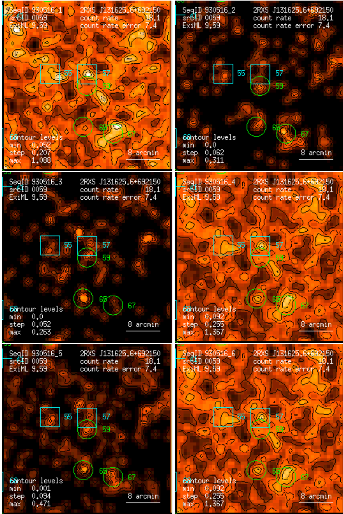
Figure 59: RASS 930516: detection 0059: band rate images, Gaussian filter: (1) PSPC channels 11 – 41, (2) 52 – 90, (3) 91 – 201, (4) 11 – 235, (5) 52 – 201, (6) 11 – 201. Broad band rates in counts/ks. Band rate contour levels in counts/ks/arcmin 2 .
