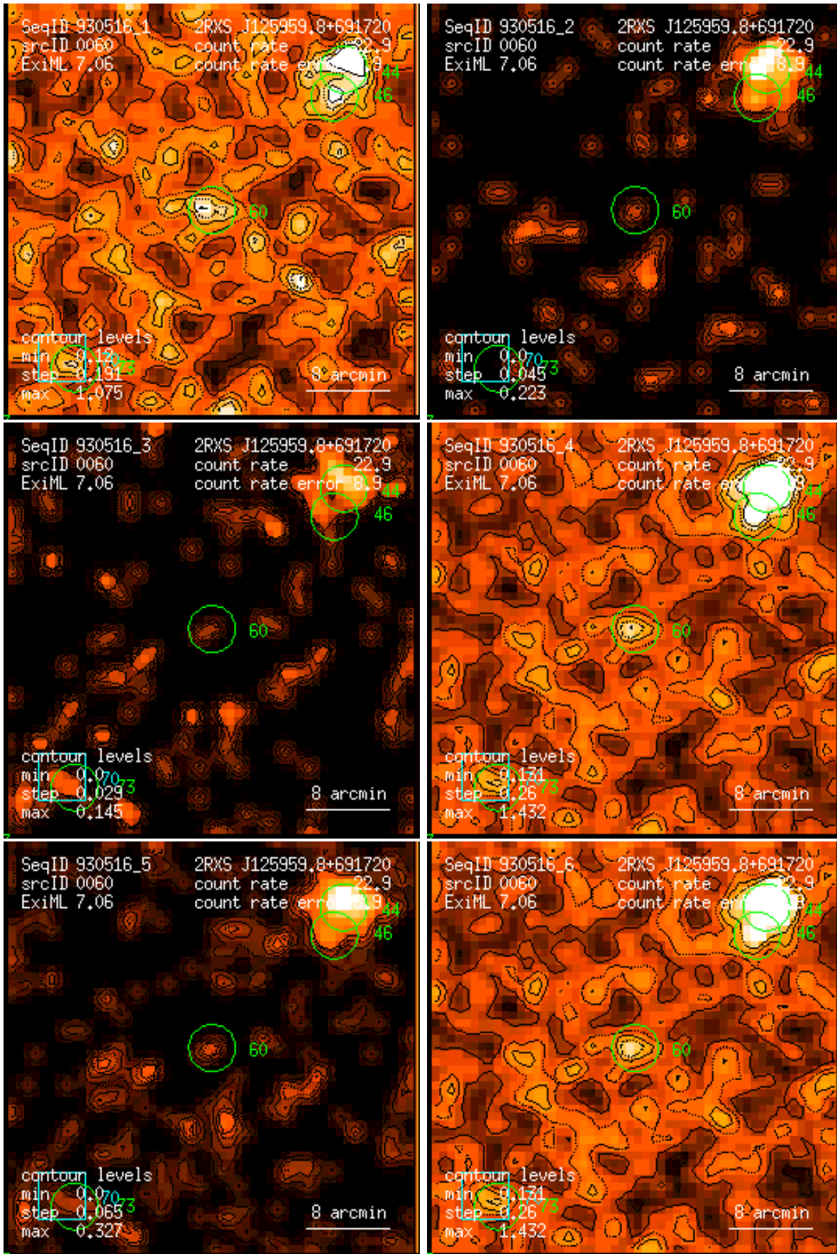
Figure 60: RASS 930516: detection 0060: band rate images, Gaussian filter: (1) PSPC channels 11 – 41, (2) 52 – 90, (3) 91 – 201, (4) 11 – 235, (5) 52 – 201, (6) 11 – 201. Broad band rates in counts/ks. Band rate contour levels in counts/ks/arcmin 2 .
