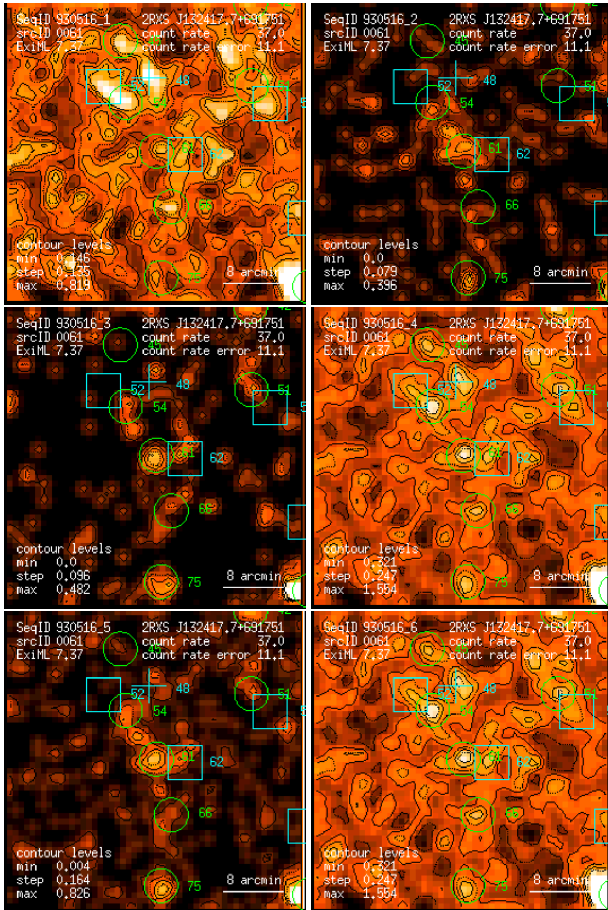
Figure 61: RASS 930516: detection 0061: band rate images, Gaussian filter: (1) PSPC channels 11 – 41, (2) 52 – 90, (3) 91 – 201, (4) 11 – 235, (5) 52 – 201, (6) 11 – 201. Broad band rates in counts/ks. Band rate contour levels in counts/ks/arcmin 2 .
