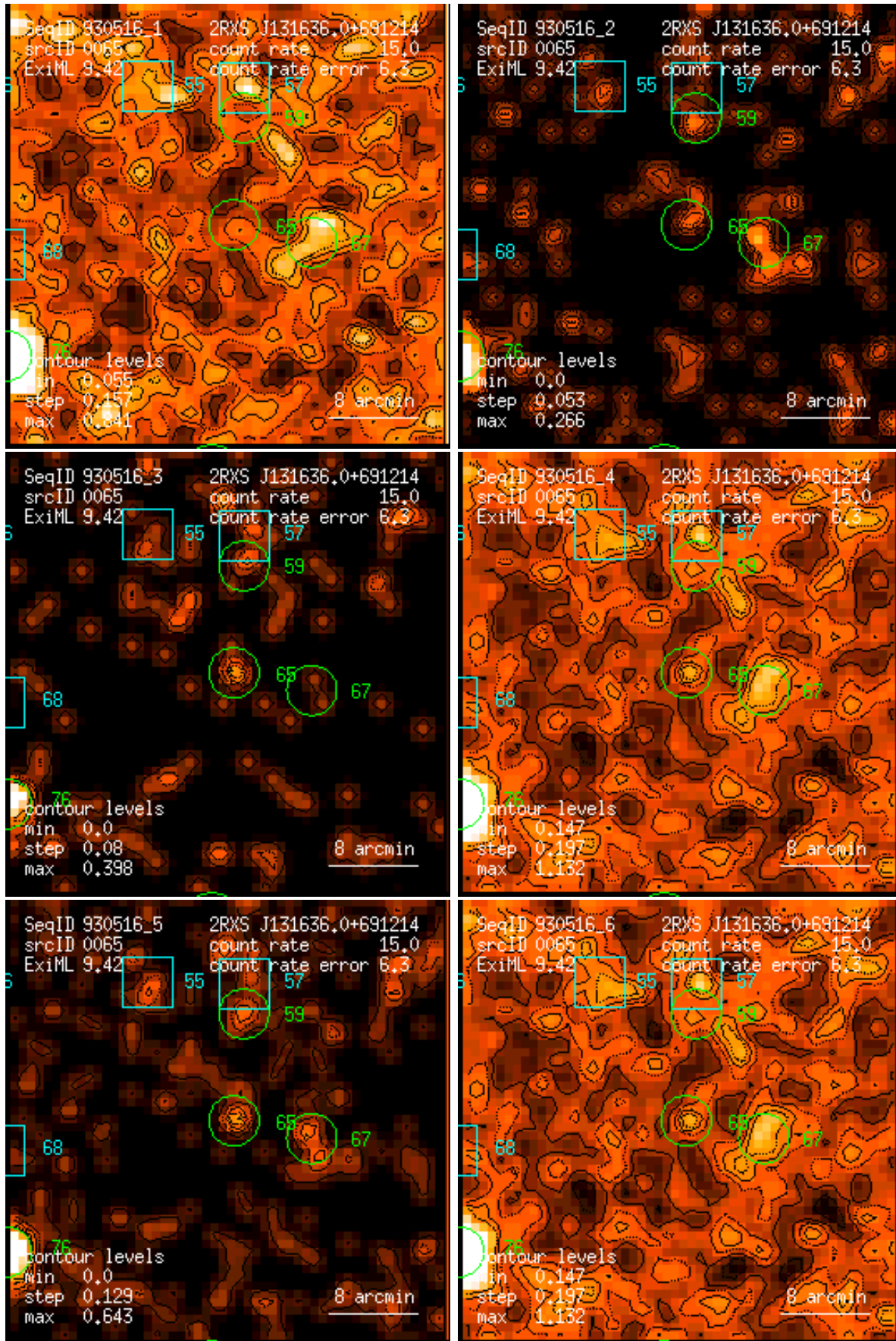
Figure 65: RASS 930516: detection 0065: band rate images, Gaussian filter: (1) PSPC channels 11 – 41, (2) 52 – 90, (3) 91 – 201, (4) 11 – 235, (5) 52 – 201, (6) 11 – 201. Broad band rates in counts/ks. Band rate contour levels in counts/ks/arcmin 2 .
