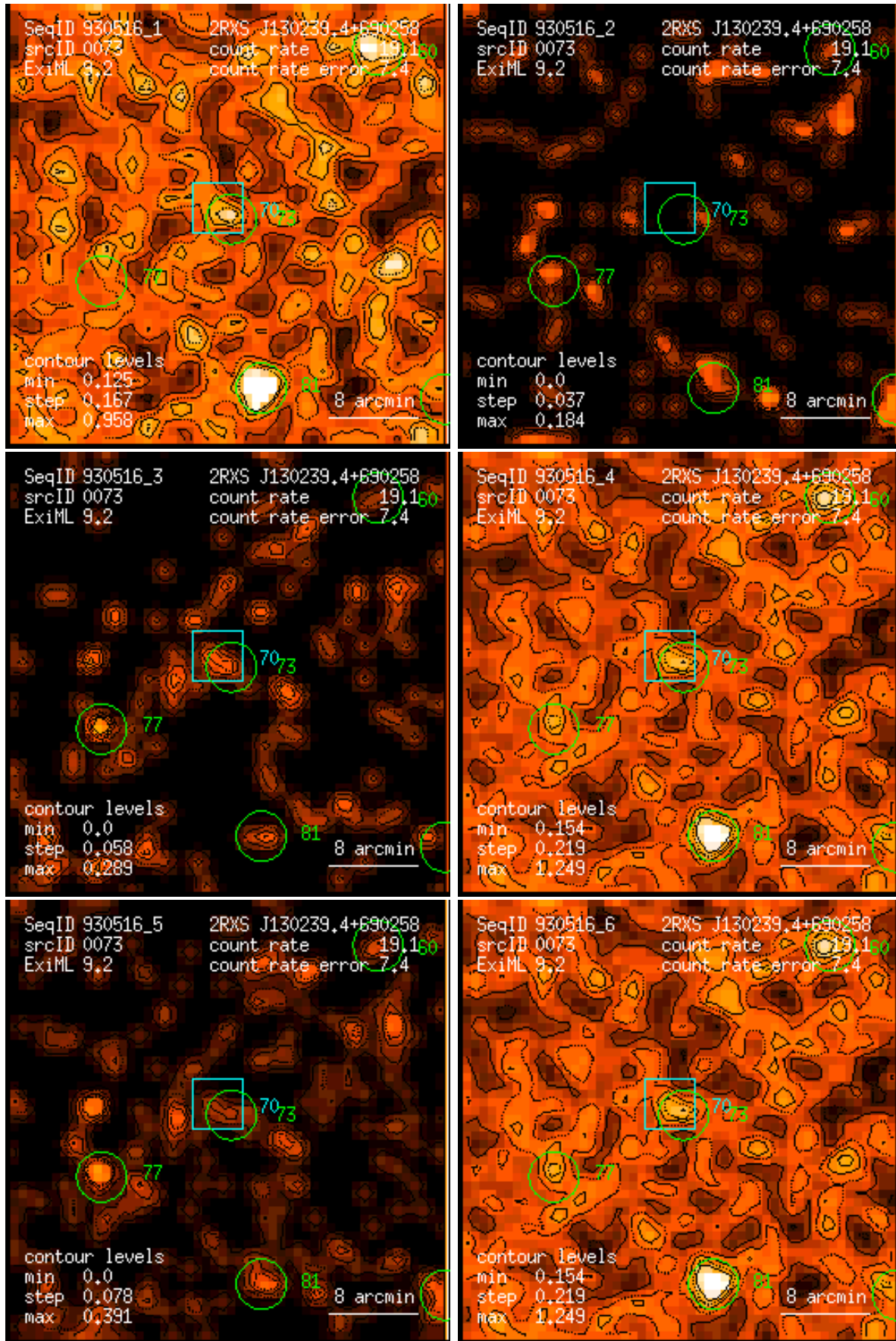
Figure 73: RASS 930516: detection 0073: band rate images, Gaussian filter: (1) PSPC channels 11 – 41, (2) 52 – 90, (3) 91 – 201, (4) 11 – 235, (5) 52 – 201, (6) 11 – 201. Broad band rates in counts/ks. Band rate contour levels in counts/ks/arcmin 2 .
