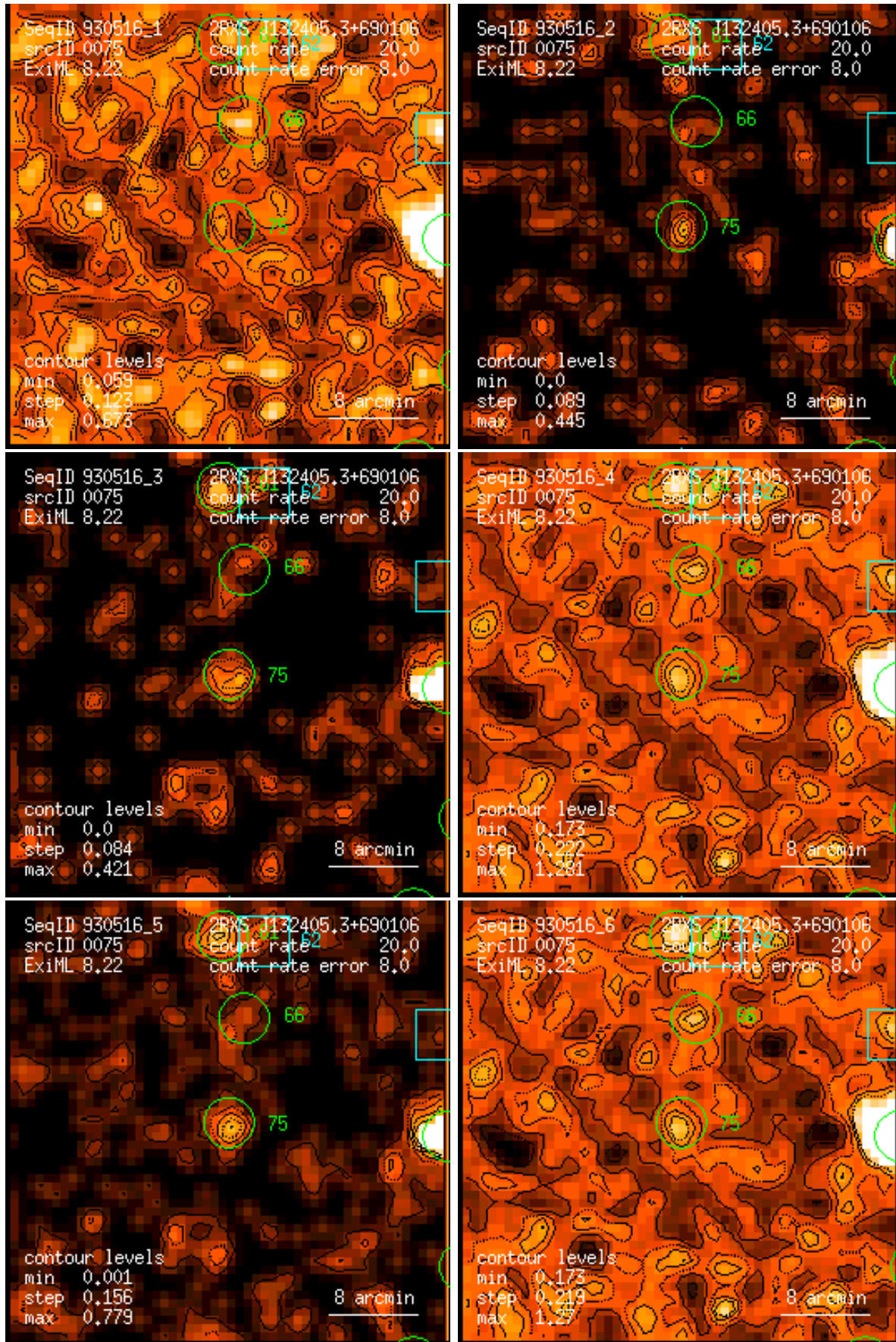
Figure 75: RASS 930516: detection 0075: band rate images, Gaussian filter: (1) PSPC channels 11 – 41, (2) 52 – 90, (3) 91 – 201, (4) 11 – 235, (5) 52 – 201, (6) 11 – 201. Broad band rates in counts/ks. Band rate contour levels in counts/ks/arcmin 2 .
