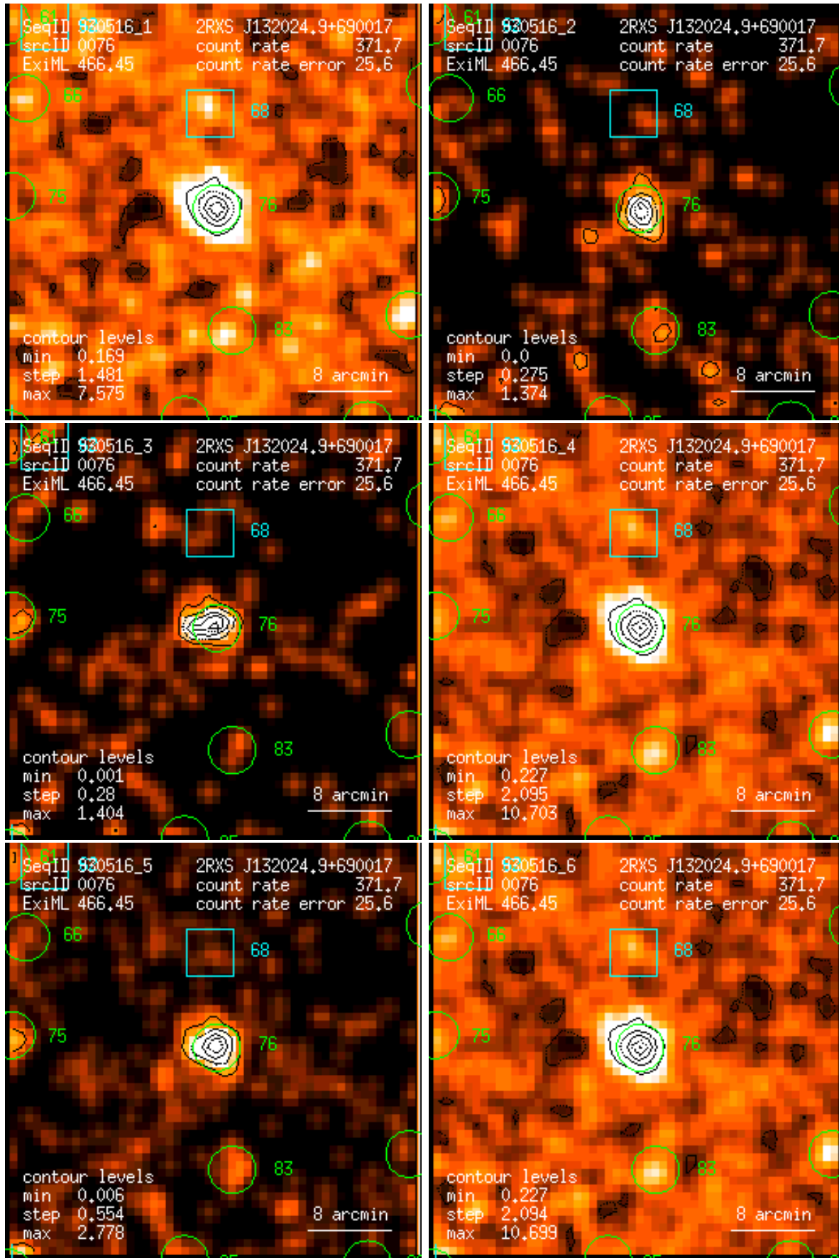
Figure 76: RASS 930516: detection 0076: band rate images, Gaussian filter: (1) PSPC channels 11 – 41, (2) 52 – 90, (3) 91 – 201, (4) 11 – 235, (5) 52 – 201, (6) 11 – 201. Broad band rates in counts/ks. Band rate contour levels in counts/ks/arcmin 2 .
