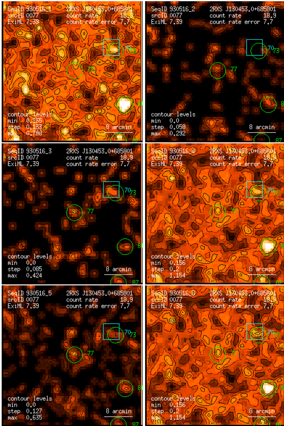
Figure 77: RASS 930516: detection 0077: band rate images, Gaussian filter: (1) PSPC channels 11 – 41, (2) 52 – 90, (3) 91 – 201, (4) 11 – 235, (5) 52 – 201, (6) 11 – 201. Broad band rates in counts/ks. Band rate contour levels in counts/ks/arcmin 2 .
