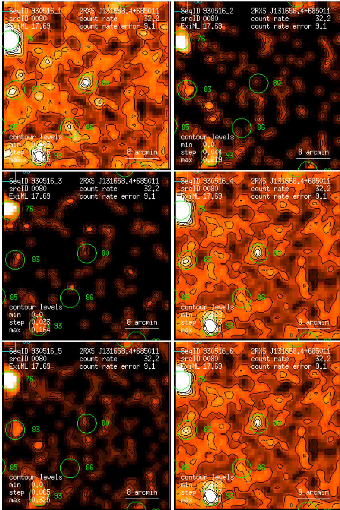
Figure 80: RASS 930516: detection 0080: band rate images, Gaussian filter: (1) PSPC channels 11 – 41, (2) 52 – 90, (3) 91 – 201, (4) 11 – 235, (5) 52 – 201, (6) 11 – 201. Broad band rates in counts/ks. Band rate contour levels in counts/ks/arcmin 2 .
