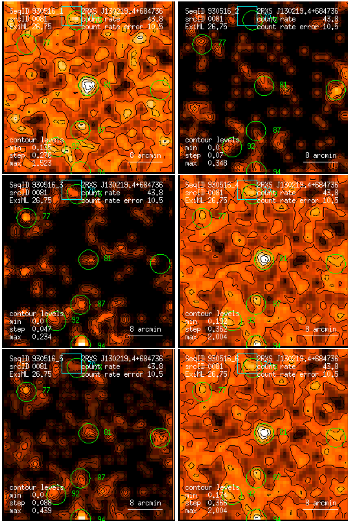
Figure 81: RASS 930516: detection 0081: band rate images, Gaussian filter: (1) PSPC channels 11 – 41, (2) 52 – 90, (3) 91 – 201, (4) 11 – 235, (5) 52 – 201, (6) 11 – 201. Broad band rates in counts/ks. Band rate contour levels in counts/ks/arcmin 2 .
