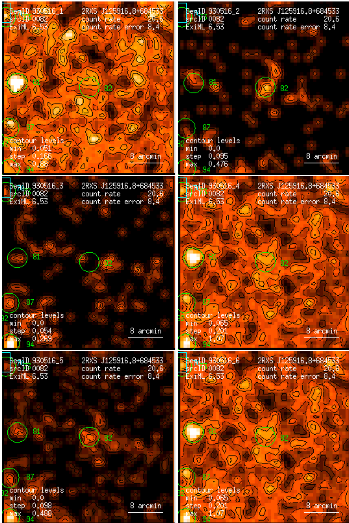
Figure 82: RASS 930516: detection 0082: band rate images, Gaussian filter: (1) PSPC channels 11 – 41, (2) 52 – 90, (3) 91 – 201, (4) 11 – 235, (5) 52 – 201, (6) 11 – 201. Broad band rates in counts/ks. Band rate contour levels in counts/ks/arcmin 2 .
