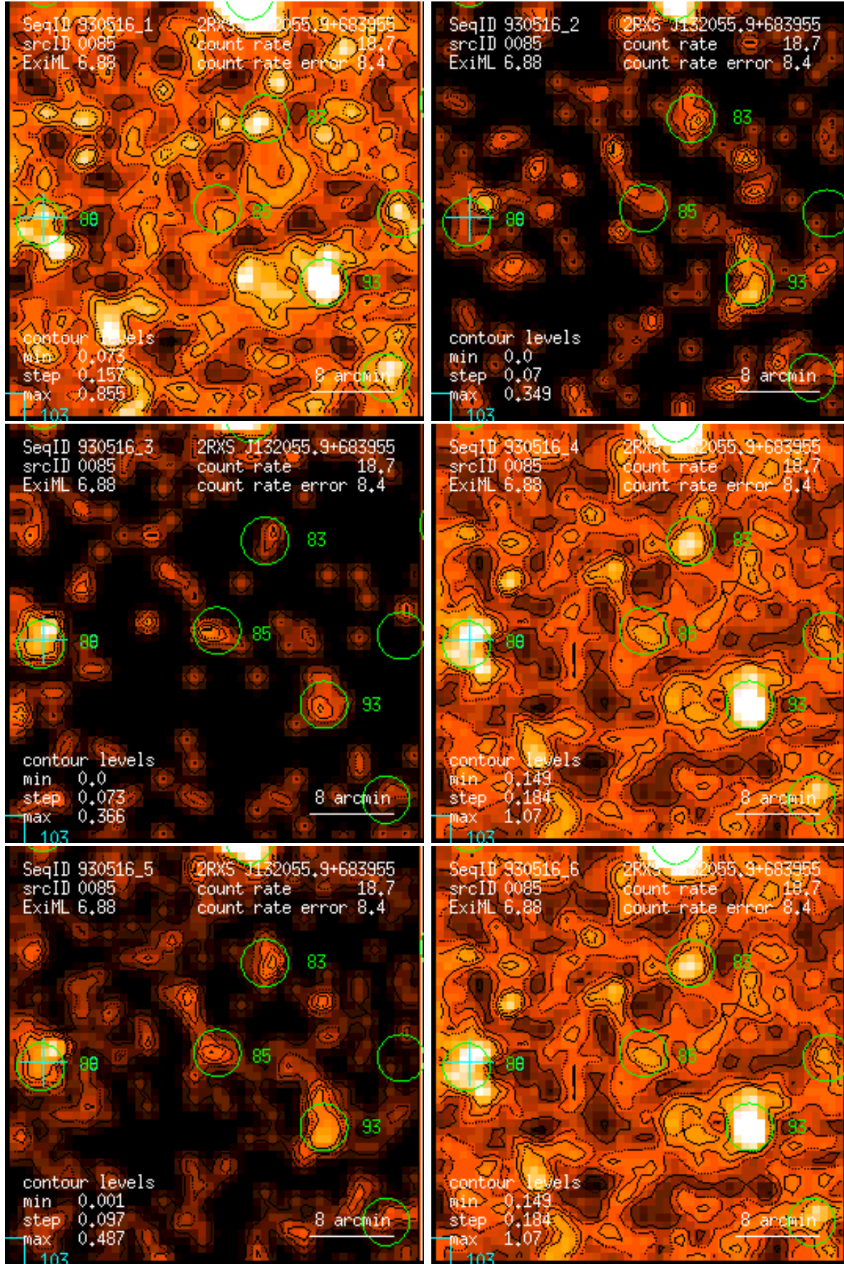
Figure 85: RASS 930516: detection 0085: band rate images, Gaussian filter: (1) PSPC channels 11 – 41, (2) 52 – 90, (3) 91 – 201, (4) 11 – 235, (5) 52 – 201, (6) 11 – 201. Broad band rates in counts/ks. Band rate contour levels in counts/ks/arcmin 2 .
