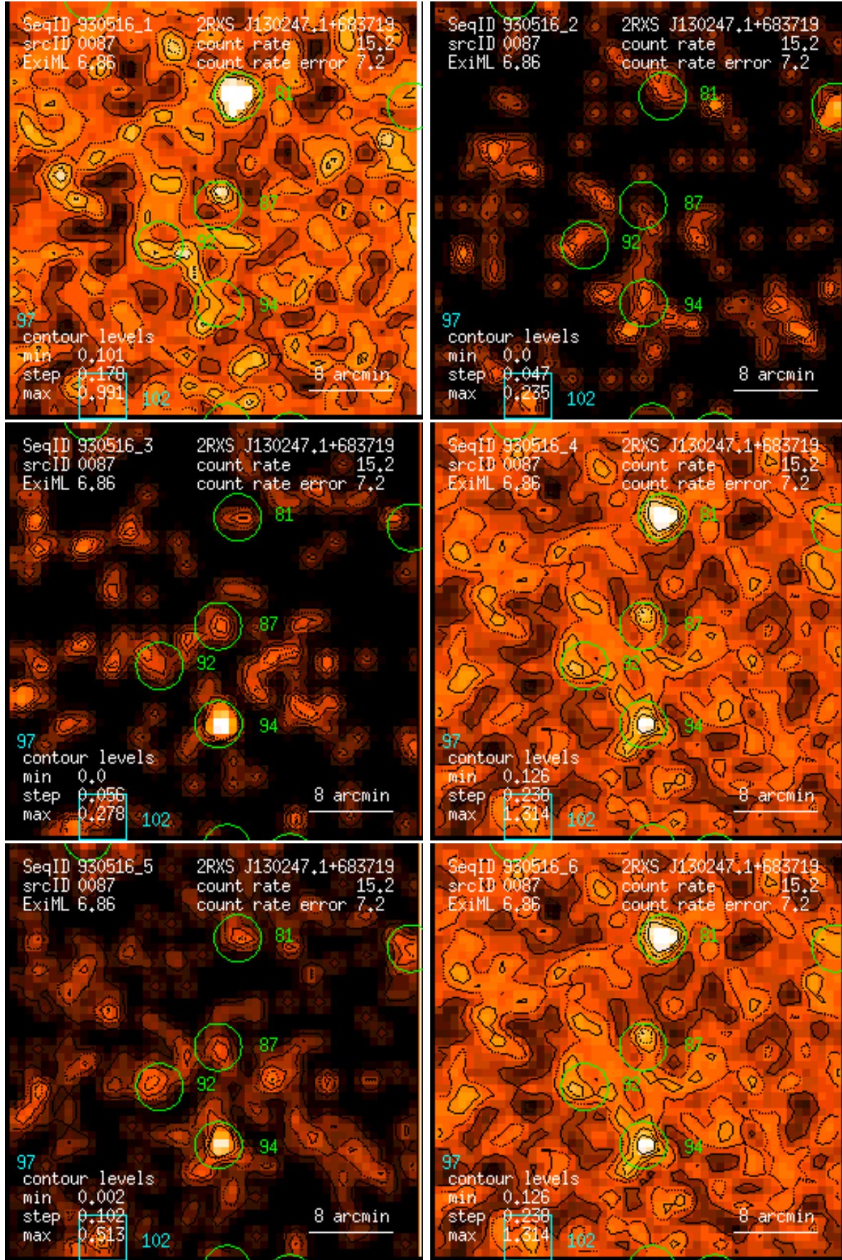
Figure 87: RASS 930516: detection 0087: band rate images, Gaussian filter: (1) PSPC channels 11 – 41, (2) 52 – 90, (3) 91 – 201, (4) 11 – 235, (5) 52 – 201, (6) 11 – 201. Broad band rates in counts/ks. Band rate contour levels in counts/ks/arcmin 2 .
