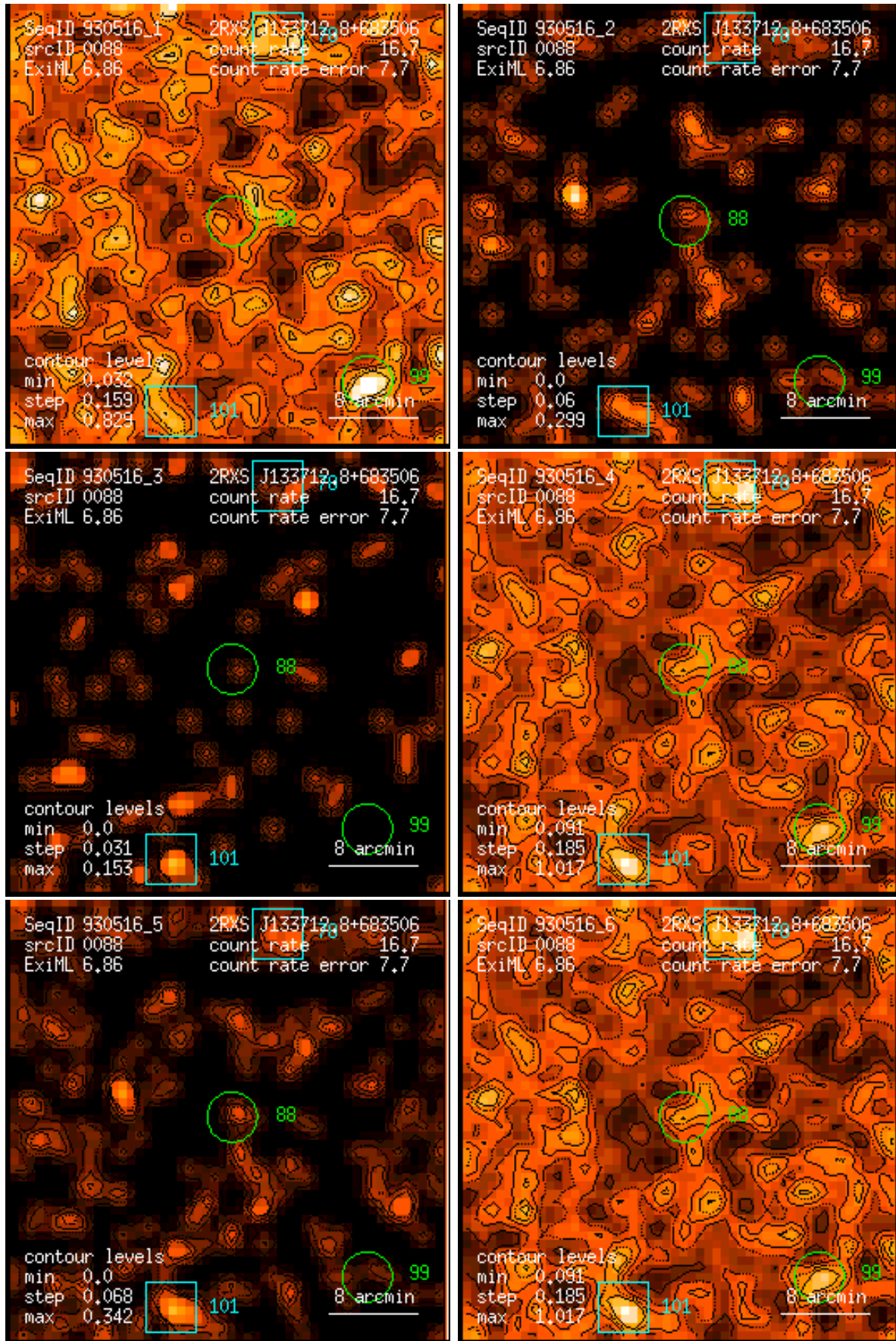
Figure 88: RASS 930516: detection 0088: band rate images, Gaussian filter: (1) PSPC channels 11 – 41, (2) 52 – 90, (3) 91 – 201, (4) 11 – 235, (5) 52 – 201, (6) 11 – 201. Broad band rates in counts/ks. Band rate contour levels in counts/ks/arcmin 2 .
