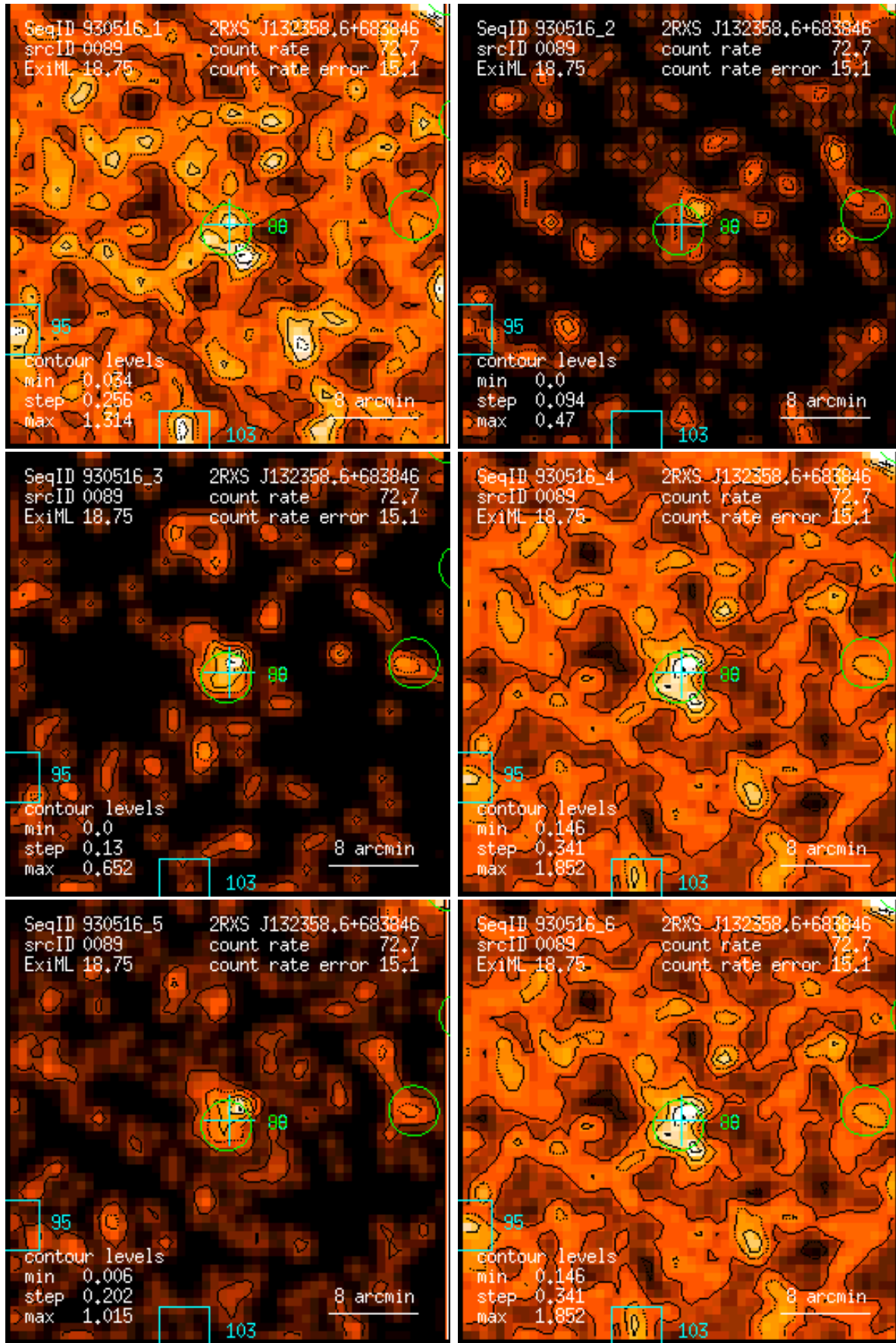
Figure 89: RASS 930516: detection 0089: band rate images, Gaussian filter: (1) PSPC channels 11 – 41, (2) 52 – 90, (3) 91 – 201, (4) 11 – 235, (5) 52 – 201, (6) 11 – 201. Broad band rates in counts/ks. Band rate contour levels in counts/ks/arcmin 2 .
