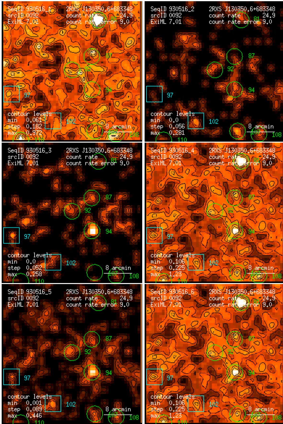
Figure 92: RASS 930516: detection 0092: band rate images, Gaussian filter: (1) PSPC channels 11 – 41, (2) 52 – 90, (3) 91 – 201, (4) 11 – 235, (5) 52 – 201, (6) 11 – 201. Broad band rates in counts/ks. Band rate contour levels in counts/ks/arcmin 2 .
