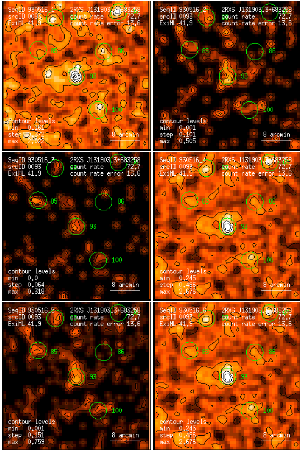
Figure 93: RASS 930516: detection 0093: band rate images, Gaussian filter: (1) PSPC channels 11 – 41, (2) 52 – 90, (3) 91 – 201, (4) 11 – 235, (5) 52 – 201, (6) 11 – 201. Broad band rates in counts/ks. Band rate contour levels in counts/ks/arcmin 2 .
