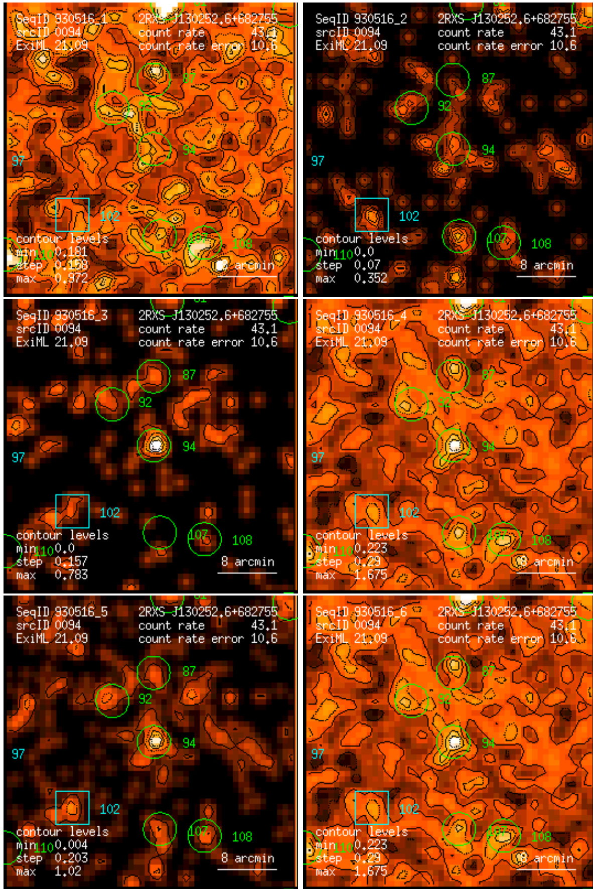
Figure 94: RASS 930516: detection 0094: band rate images, Gaussian filter: (1) PSPC channels 11 – 41, (2) 52 – 90, (3) 91 – 201, (4) 11 – 235, (5) 52 – 201, (6) 11 – 201. Broad band rates in counts/ks. Band rate contour levels in counts/ks/arcmin 2 .
