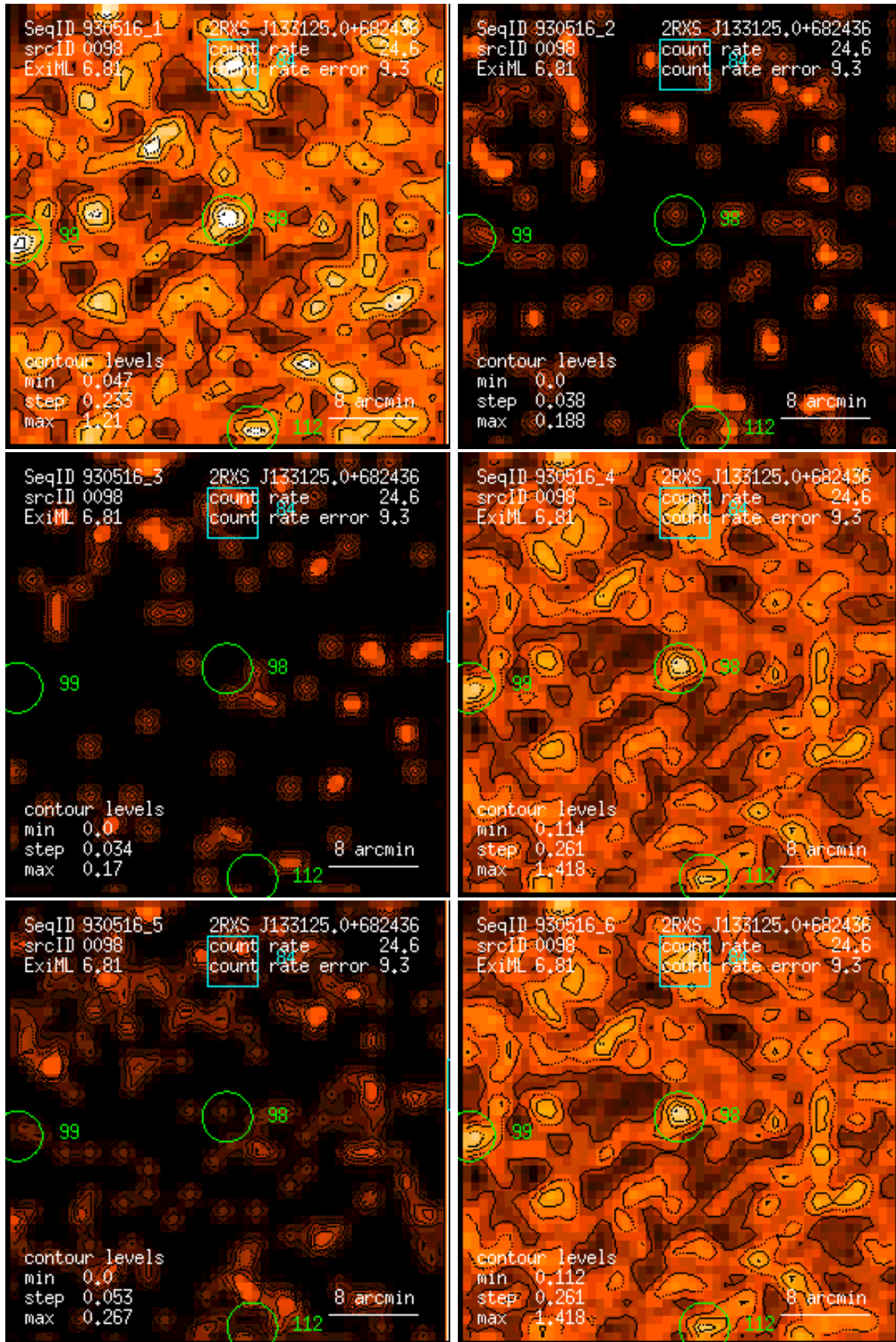
Figure 98: RASS 930516: detection 0098: band rate images, Gaussian filter: (1) PSPC channels 11 – 41, (2) 52 – 90, (3) 91 – 201, (4) 11 – 235, (5) 52 – 201, (6) 11 – 201. Broad band rates in counts/ks. Band rate contour levels in counts/ks/arcmin 2 .
