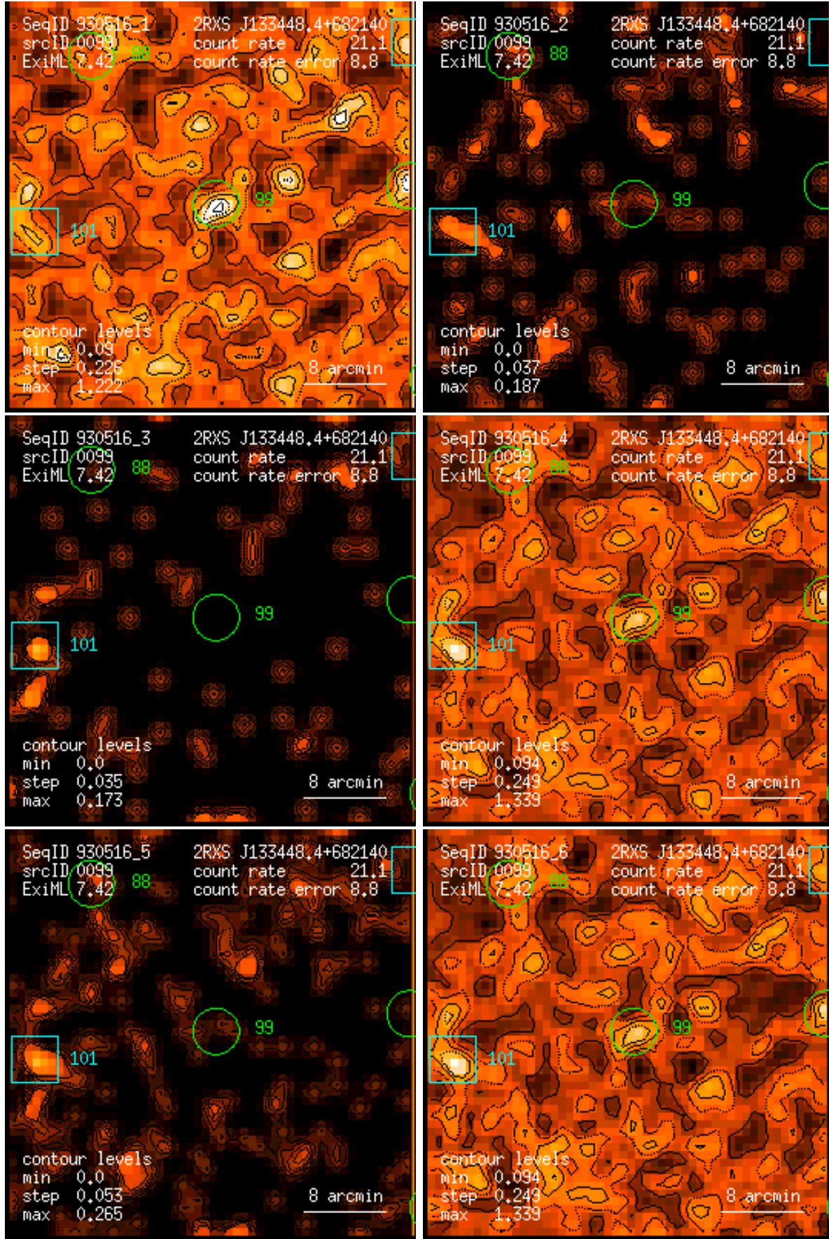
Figure 99: RASS 930516: detection 0099: band rate images, Gaussian filter: (1) PSPC channels 11 – 41, (2) 52 – 90, (3) 91 – 201, (4) 11 – 235, (5) 52 – 201, (6) 11 – 201. Broad band rates in counts/ks. Band rate contour levels in counts/ks/arcmin 2 .
