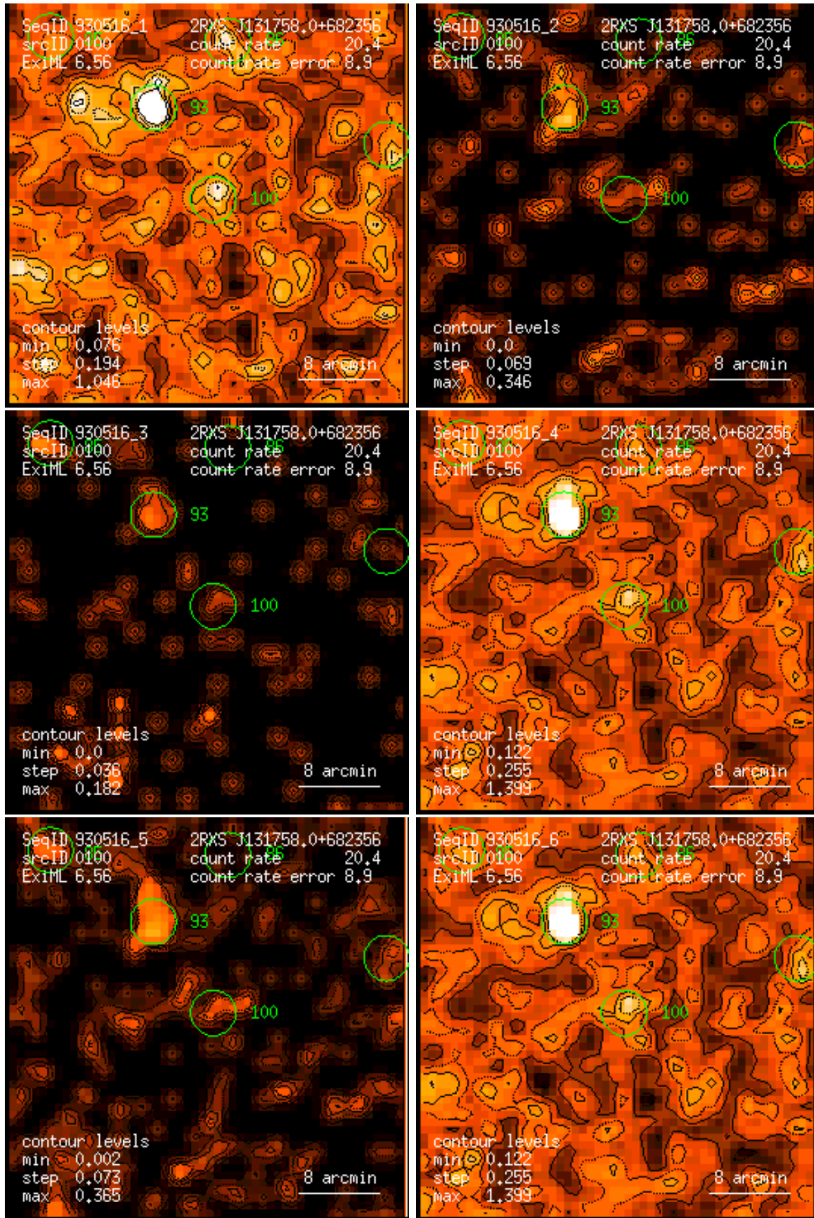
Figure 100: RASS 930516: detection 0100: band rate images, Gaussian filter: (1) PSPC channels 11 – 41, (2) 52 – 90, (3) 91 – 201, (4) 11 – 235, (5) 52 – 201, (6) 11 – 201. Broad band rates in counts/ks. Band rate contour levels in counts/ks/arcmin 2 .
