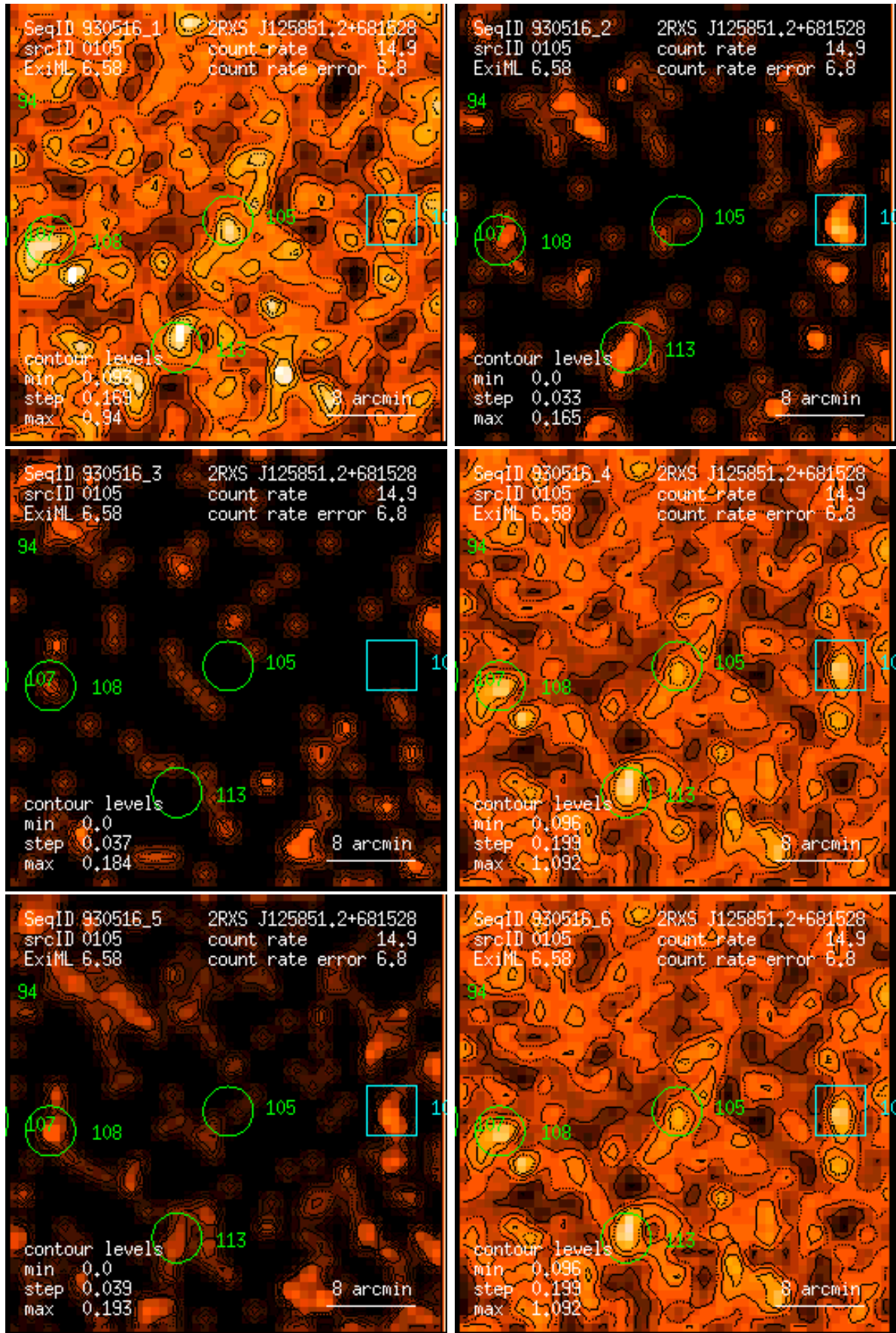
Figure 105: RASS 930516: detection 0105: band rate images, Gaussian filter: (1) PSPC channels 11 – 41, (2) 52 – 90, (3) 91 – 201, (4) 11 – 235, (5) 52 – 201, (6) 11 – 201. Broad band rates in counts/ks. Band rate contour levels in counts/ks/arcmin 2 .
