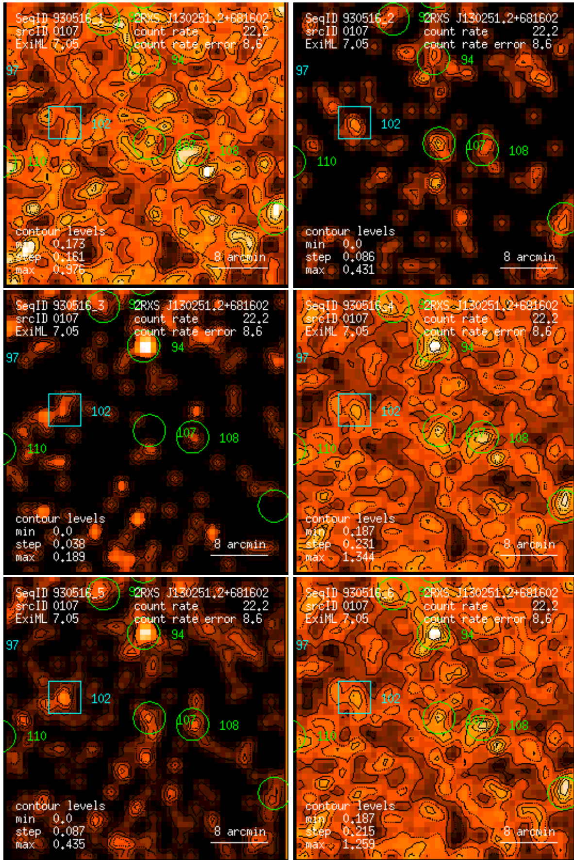
Figure 107: RASS 930516: detection 0107: band rate images, Gaussian filter: (1) PSPC channels 11 – 41, (2) 52 – 90, (3) 91 – 201, (4) 11 – 235, (5) 52 – 201, (6) 11 – 201. Broad band rates in counts/ks. Band rate contour levels in counts/ks/arcmin 2 .
