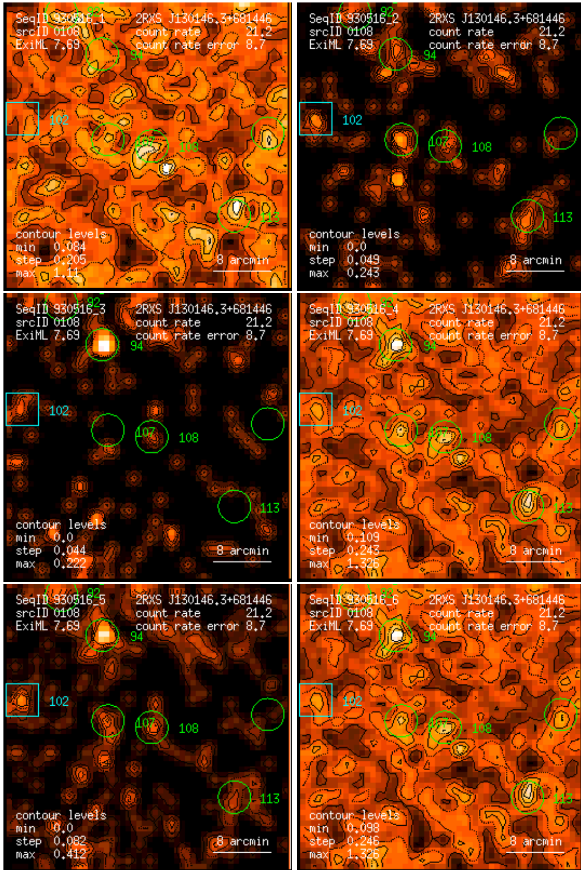
Figure 108: RASS 930516: detection 0108: band rate images, Gaussian filter: (1) PSPC channels 11 – 41, (2) 52 – 90, (3) 91 – 201, (4) 11 – 235, (5) 52 – 201, (6) 11 – 201. Broad band rates in counts/ks. Band rate contour levels in counts/ks/arcmin 2 .
