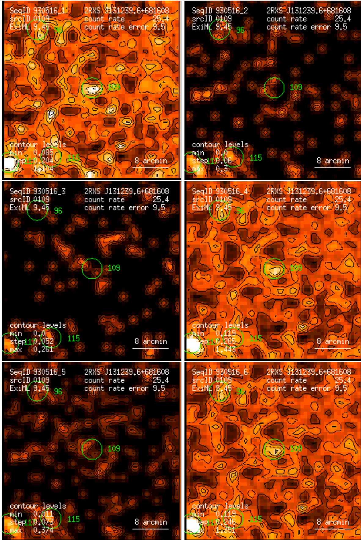
Figure 109: RASS 930516: detection 0109: band rate images, Gaussian filter: (1) PSPC channels 11 – 41, (2) 52 – 90, (3) 91 – 201, (4) 11 – 235, (5) 52 – 201, (6) 11 – 201. Broad band rates in counts/ks. Band rate contour levels in counts/ks/arcmin 2 .
