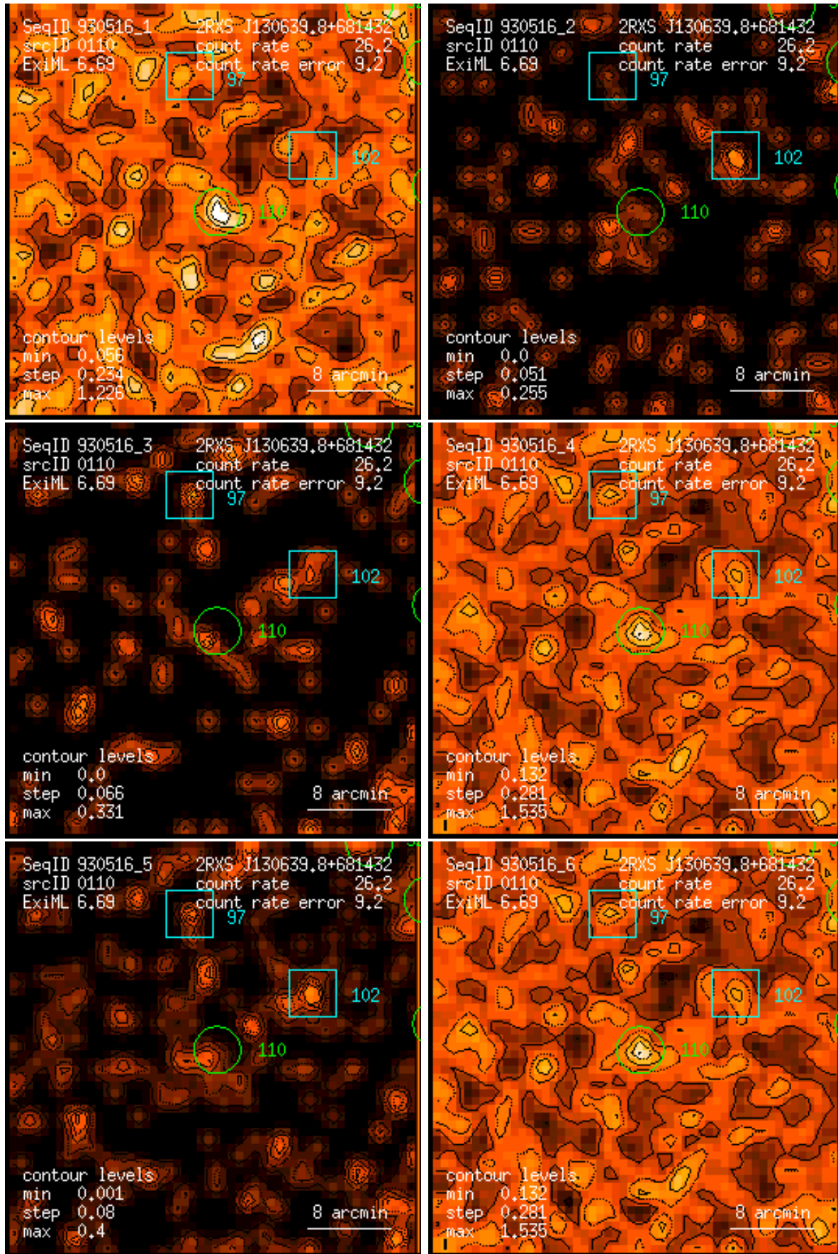
Figure 110: RASS 930516: detection 0110: band rate images, Gaussian filter: (1) PSPC channels 11 – 41, (2) 52 – 90, (3) 91 – 201, (4) 11 – 235, (5) 52 – 201, (6) 11 – 201. Broad band rates in counts/ks. Band rate contour levels in counts/ks/arcmin 2 .
