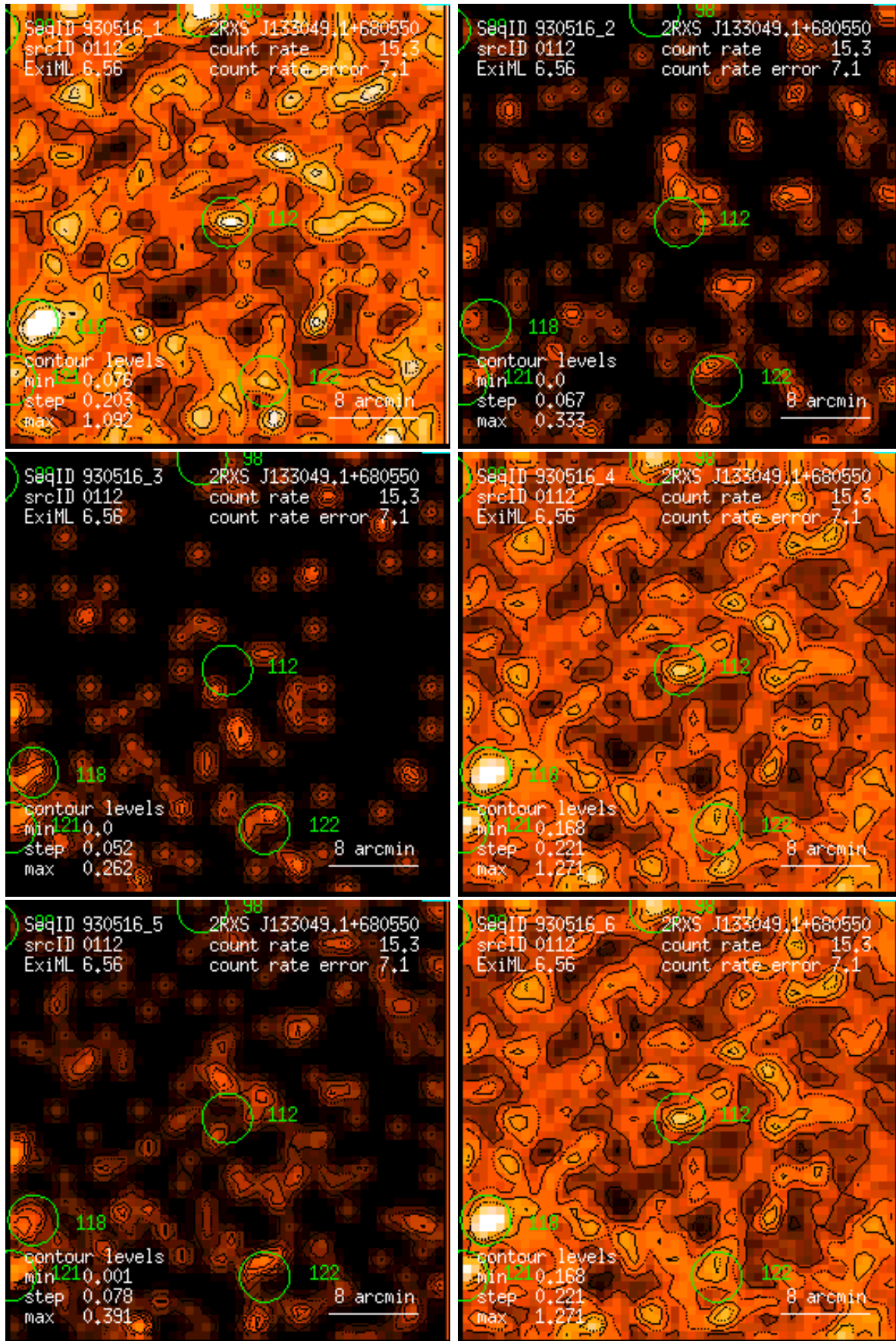
Figure 112: RASS 930516: detection 0112: band rate images, Gaussian filter: (1) PSPC channels 11 – 41, (2) 52 – 90, (3) 91 – 201, (4) 11 – 235, (5) 52 – 201, (6) 11 – 201. Broad band rates in counts/ks. Band rate contour levels in counts/ks/arcmin 2 .
