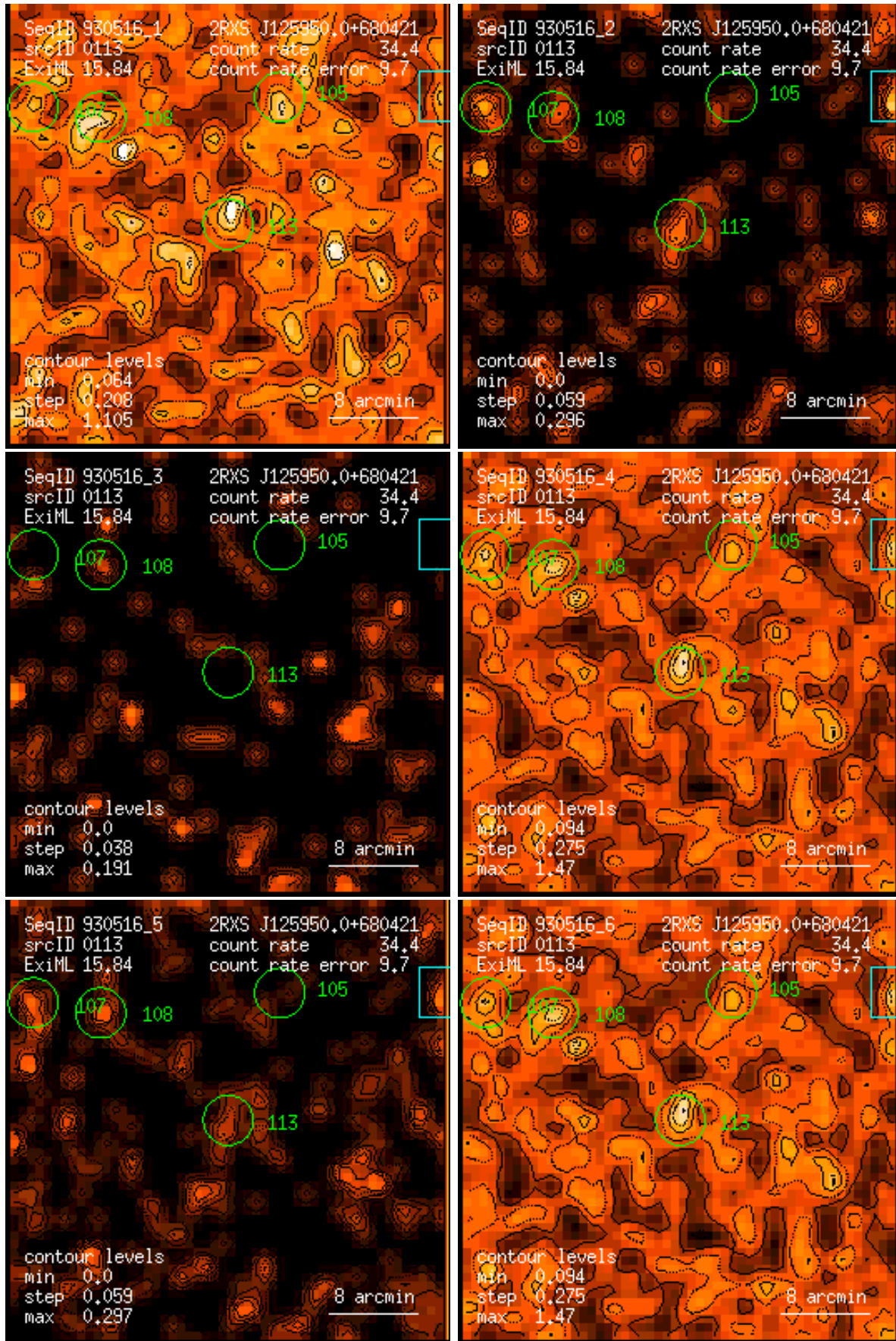
Figure 113: RASS 930516: detection 0113: band rate images, Gaussian filter: (1) PSPC channels 11 – 41, (2) 52 – 90, (3) 91 – 201, (4) 11 – 235, (5) 52 – 201, (6) 11 – 201. Broad band rates in counts/ks. Band rate contour levels in counts/ks/arcmin 2 .
