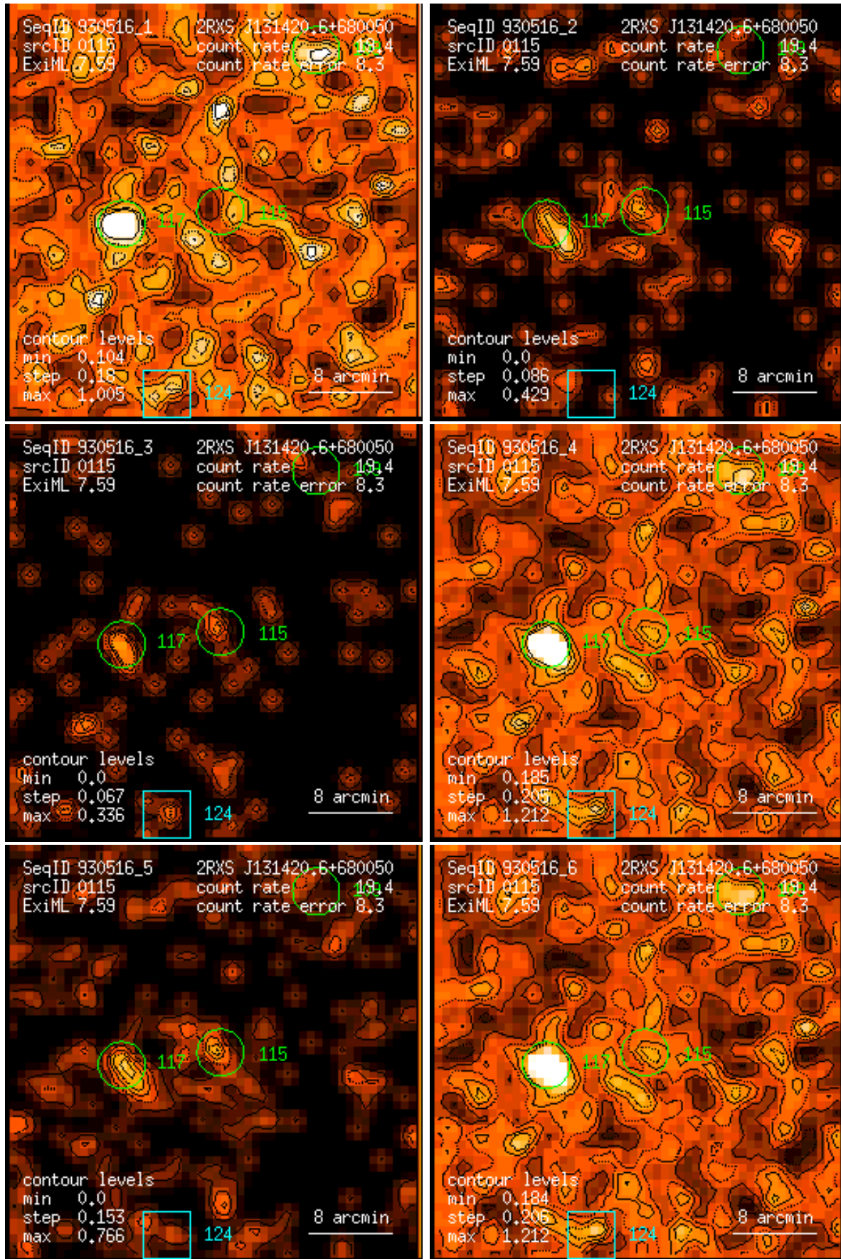
Figure 115: RASS 930516: detection 0115: band rate images, Gaussian filter: (1) PSPC channels 11 – 41, (2) 52 – 90, (3) 91 – 201, (4) 11 – 235, (5) 52 – 201, (6) 11 – 201. Broad band rates in counts/ks. Band rate contour levels in counts/ks/arcmin 2 .
